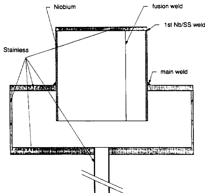
Figure 1. Test-piece for Niobium-Stainless welds
