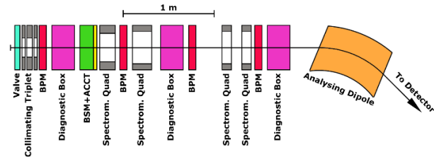
Figure 5: Schematic layout of the diagnostics testbench. The diagnostic boxes contain slits and/or grids. The sketch is longitudinally at scale.
