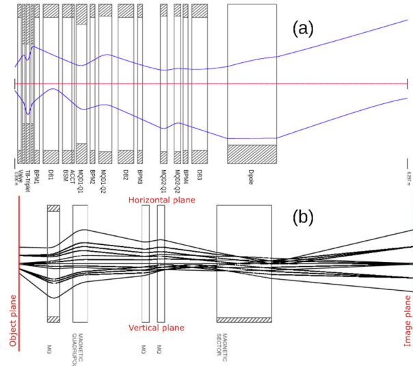
Figure 6: a) Beam envelopes in the horizontal and vertical planes, upper and lower half respectively. b) The point-to-point imaging feature of the spectrometer.
