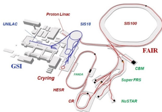
Figure 1: Layout of the FAIR facility.
