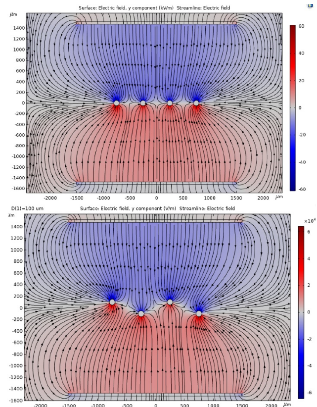
Figure 4: Field distribution calculated for co-planar wires (upper). Field distribution with alternating wire positions (lower). The diamond shaped cleaning electrodes are located at top and bottom respectively.
