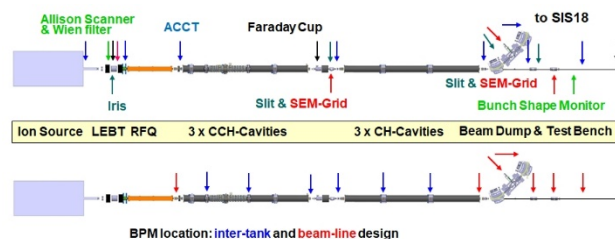
Figure 2: The FAIR proton Linac, showing the positions of the diagnostics elements (upper) and the BPMs (lower).
