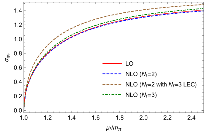
Fig. 1. \alpha_{gs} as a function of \mu_I/m_\pi at LO (red), at NLO with two flavors (blue), NLO with three flavors (green), and NLO with two flavors and three-flavor LECs (brown). See main text for details.
