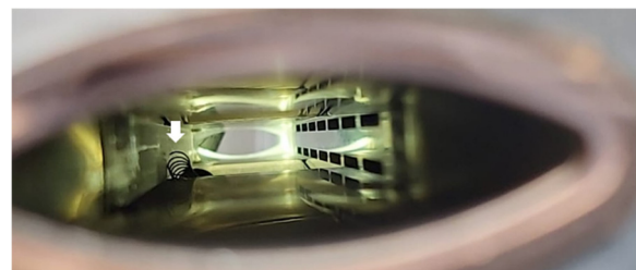
Figure 7: Vertical scraper with the coil spring that popped up in front of the beam path.
