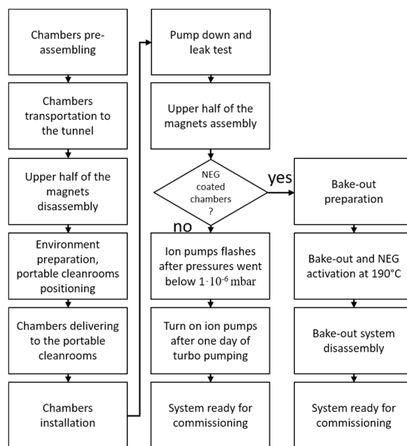
Figure 1: Vacuum installation process flow chart.
