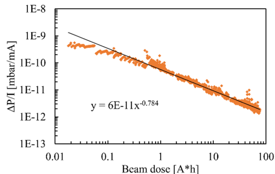
Figure 5: Normalized average dynamic pressure rise ( \Delta P/I ) as function of the beam dose.
