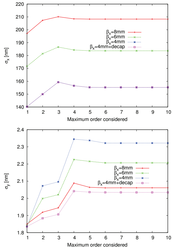
Figure 3: High order optimization using MAPCLASS for CLIC FFS for horizontal plane (top) and vertical plane (bottom).
