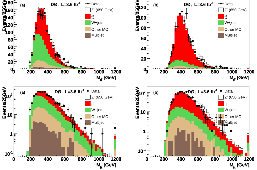
Figure 7.1: Expected and observed t\bar{t} invariant mass distribution for the combined \ell + 3\text{jets} , and \ell + 4 or more jets channels, with at least one identified b -jet. The left column (a) shows the 3-jet bin, while the right one (b) shows the 4-jet bin with at least one b -tag. The first row has a linear scale and the second a logarithmic one. The error bars for the data drawn on top of the SM background indicate the statistical uncertainty. Superimposed as white area is the theory signal for a top-color-assisted technicolor Z' boson with M_{Z'} = 650 GeV for illustration purposes. The number of data, signal and expected background events from each source are indicated in table 7.1.
