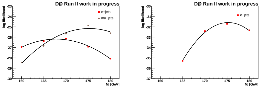
Figure A.1: Observed likelihood curves fitted with a second order polynomial for the individual \ell +jets channels in Run IIa (left) and Run IIb (right).
