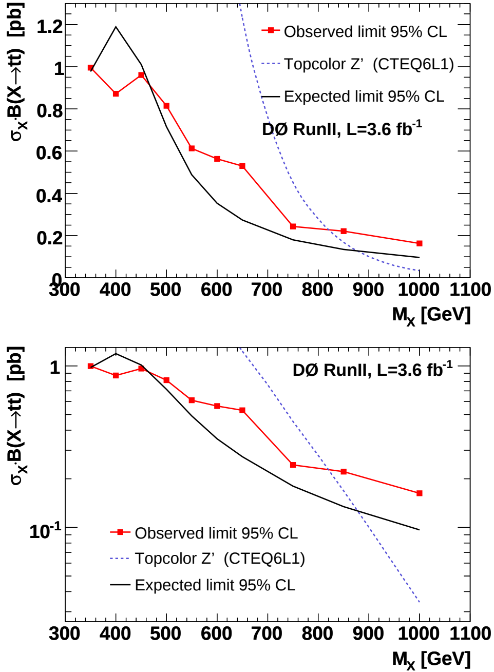
Figure 7.6: Expected and observed \sigma_X \times B(X \rightarrow t\bar{t}) obtained in 3.6 fb -1 . The black curve shows the 95% expected exclusion region, while the red curve shows the corresponding observed 95% C.L. upper limits. The theoretical prediction for a top-color-assisted technicolor Z' boson with a width of \Gamma_{Z'} = 0.012M_{Z'} as a function of the resonance mass M_X is shown as a dashed line. The upper figure shows the linear plots, while the lower one features a logarithmic cross section axis.
