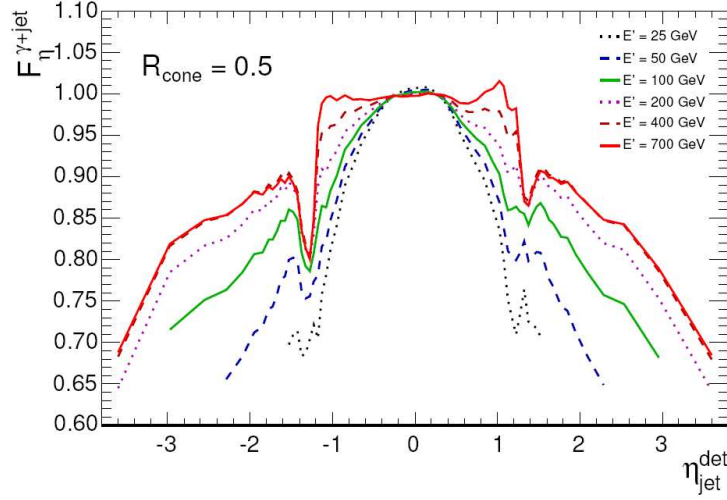
Figure 4.7: Relative response correction for JES in data [118]. The correction factor F_{\eta} is shown depending on the jet \eta . A low value means a low response from the calorimeter, as the factor is in the denominator of the final correction. The low response in the ICD region is clearly visible.
