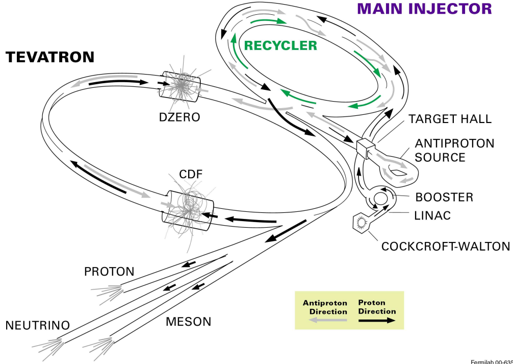
Figure 3.1: Accelerator chain [76].
