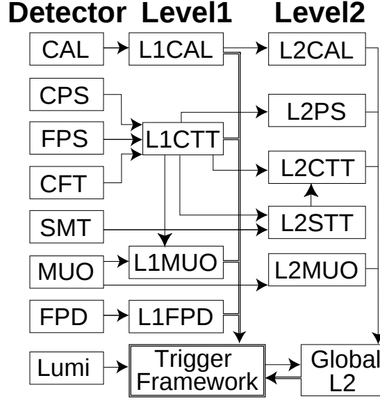
Figure 3.12: Overview of the DØ trigger and data acquisition systems [86].
