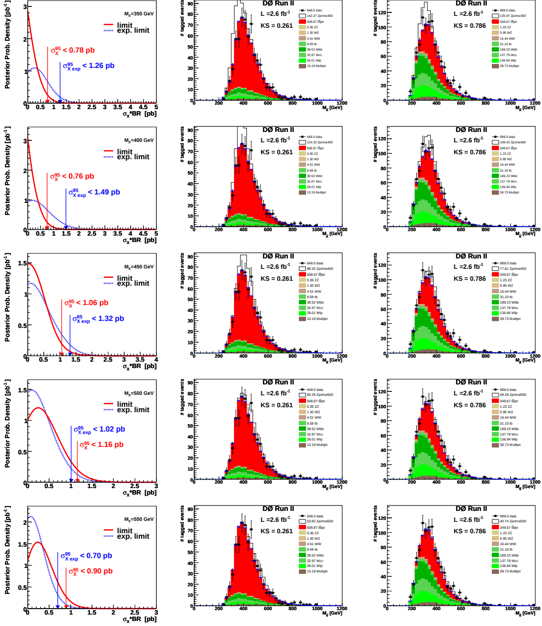
Figure 7.9: In the left plots, the posterior probability densities are shown as a function of \sigma_X \times B(X \rightarrow t\bar{t}) . M_{\tilde{t}\tilde{t}} is shown with an assumed resonance contribution in the four or more jet distribution (middle) and the 3-jet distribution (right). Each row corresponds to a different resonance mass assumption, starting from 350 GeV (top) to 550 GeV (bottom) from Run IIb.
