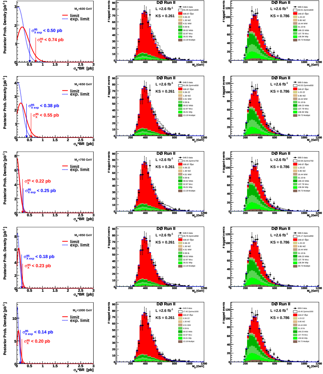
Figure 7.10: In the left plots, the posterior probability densities are shown as a function of \sigma_X \times B(X \rightarrow t\bar{t}) . M_{\tilde{t}\tilde{t}} is shown with an assumed resonance contribution in the four or more jet distribution (middle) and the 3-jet distribution (right). Each row corresponds to a different resonance mass assumption, starting from 600 GeV (top) to 1000 GeV (bottom) from Run IIb.
