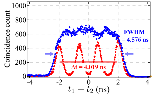
Fig. 7. Experimental results for defining the amount of dispersion in the DWDM GVD module over 1 hour. The data represented by the blue dots corresponds to the coincidence count of entangled photon pairs with the fiber spool in the idler path. The data shown in red represents the coincidence count after adding the same-length DWDM module in the signal path.
