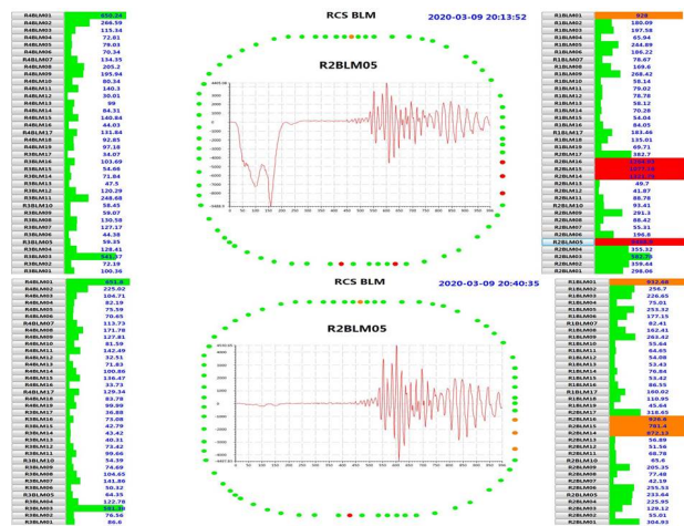
Figure 5: R2BLM05 beam loss optimization. Upper: the waveform of the R2BLM05 before correction; Bottom: the waveform of the R2BLM05 after correction.
