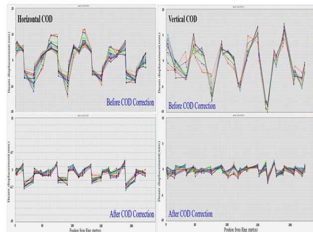
Figure 1: Global orbit corrections applied at CSNS/RCS. Upper: 20 traces of the horizontal/vertical orbit before correction. Bottom: 20 traces of the horizontal/vertical orbits after correction.
