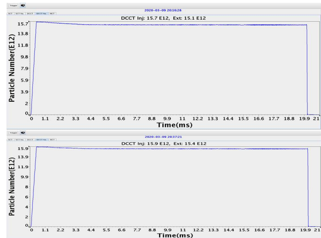
Figure 6: The comparison of the transmission rate of the RCS. Upper: the transmission rate is around 96.18% before correction; Bottom: the transmission rate is around 96.86% after correction.
