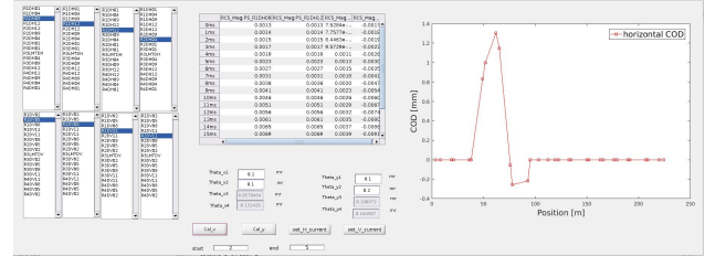
Figure 3: Local orbit correction APP developed for CSNS/RCS commissioning.
