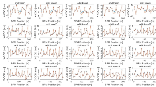
Figure 4: The horizontal orbits for 20 traces. The red circle represents the orbits before correction and the blue square represents the orbits after correction.
