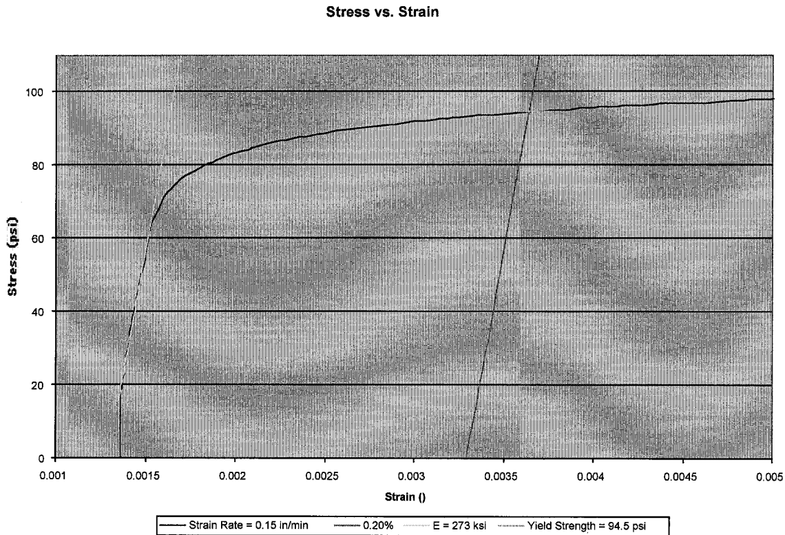
Figure 1 – Typical Stress-Strain curve
