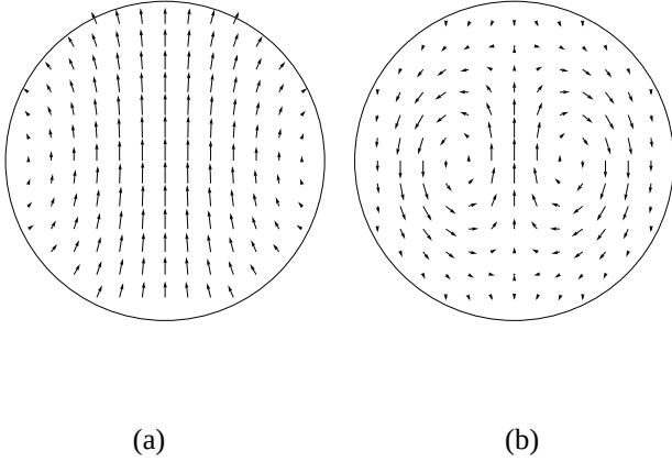
Figure 1: Cross section of transverse electric field in (a) TE_{11} and (b) TE_{12} modes in a circular waveguide.
