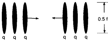
Fig. 14. The ultimate central proton-proton collision.
