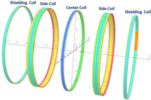
Fig. 2 The HPgTPC detector superconducting coils configuration.
