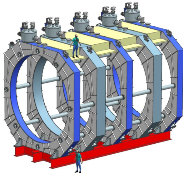
Fig. 1 HPgTPC detector magnet system overview.
