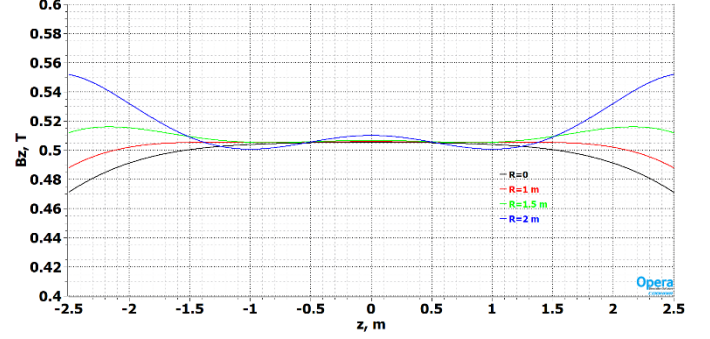
Fig. 3 Magnetic field in the magnet bore.
