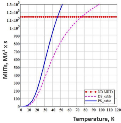
Fig. 5 Superconducting cables adiabatic heating during quench.
