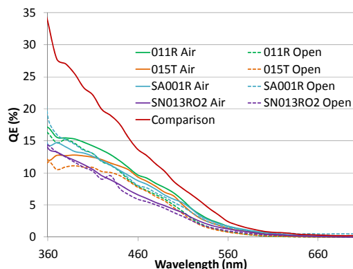
Figure 2: Spectral response of Photonis K_2CsSb photocathodes before (air) and after (open) cap removal.
