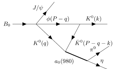
Fig. 2. Feynman diagrams of the decay process B_0 \rightarrow J/\psi K^0 a_0(980) \rightarrow J/\psi K^0 \pi^0 \eta involving a triangle loop.
