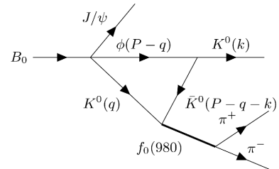
Fig. 1. Feynman diagrams of the decay process B_0 \rightarrow J/\psi K^0 f_0(980) \rightarrow J/\psi K^0 \pi^+ \pi^- involving a triangle loop.
