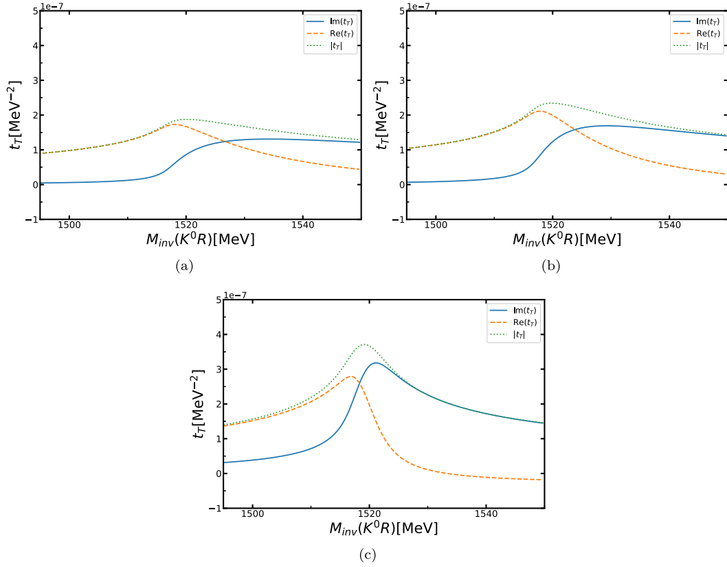
Fig. 3. (color online) Triangle amplitude t_T , as a function of M_{\text{inv}}(K^0 f_0/K^0 a_0) for (a) m_{f_0(a_0)} = 986 MeV, (b) m_{f_0(a_0)} = 991 MeV, and (c) m_{f_0(a_0)} = 996 MeV. |t_T| , \text{Re}(t_T) , and \text{Im}(t_T) are plotted using green, orange, and blue curves, respectively.
