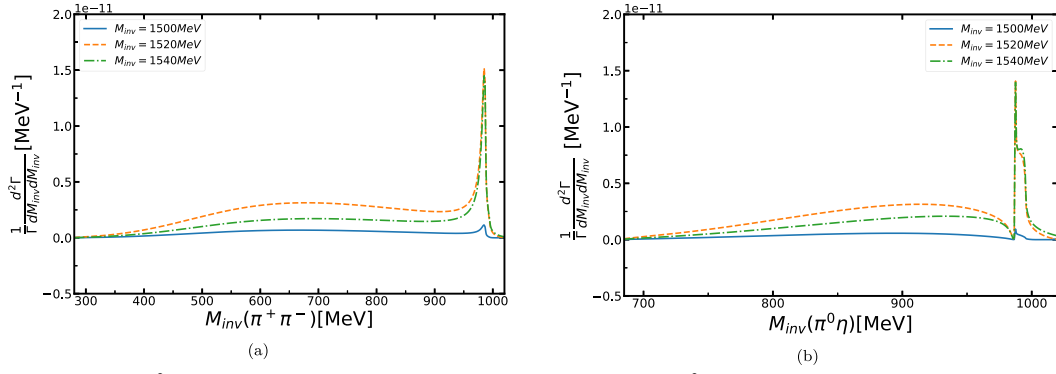
Fig. 5. (color online) (a) \frac{d^2\Gamma_{B_0 \rightarrow J/\psi K^0 f_0(980) \rightarrow \pi^+ \pi^-}}{dM_{\text{inv}}(K^0 f_0) dM_{\text{inv}}(\pi^+ \pi^-)} as a function of M_{\text{inv}}(\pi^+ \pi^-) . (b) \frac{d^2\Gamma_{B_0 \rightarrow J/\psi K^0 a_0(980) \rightarrow J/\psi K^0 \pi^0 \eta}}{dM_{\text{inv}}(K^0 a_0) dM_{\text{inv}}(\pi^0 \eta)} as a function of M_{\text{inv}}(\pi^0 \eta) . The blue, orange, and green curves are obtained by setting M_{\text{inv}}(K^0 f_0) = 1500, 1520 , and 1540 MeV, respectively.
