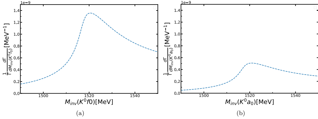
Fig. 6. (color online) (a) Differential branching ratio \frac{d\Gamma_{B_0 \rightarrow J/\psi K^0 f_0(980) \rightarrow J/\psi K^0 \pi^+ \pi^-}}{dM_{\text{inv}}(K^0 f_0)} . (b) Branching ratio \frac{d\Gamma_{B_0 \rightarrow J/\psi K^0 f_0(980) \rightarrow J/\psi K^0 \pi^+ \pi^-}}{dM_{\text{inv}}(K^0 a_0)} described in Eq. (24) as a function of M_{\text{inv}}(K^0 f_0/K^0 a_0)
