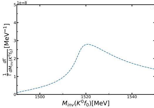
Fig. 4. (color online) Differential branching ratio \frac{1}{\Gamma_{B_0}} \frac{d\Gamma_{B_0 \rightarrow J/\psi K^0 f_0}}{dM_{\text{inv}}(K^0 f_0)} described in Eq. (23) as a function of M_{\text{inv}}(K^0 f_0/K^0 a_0)
