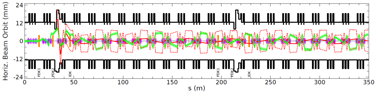
Figure 1: Trajectories of stored (green) and injected (red) particles following an injection cycle. Solid lines represent centroid, dashed lines represent 3- \sigma of the beam dimensions. The two pre-kickers and main injection kicker are labeled PDK1, PDK2, and IDK.
