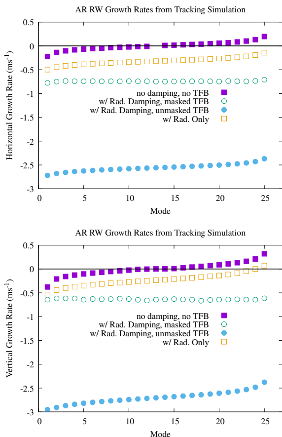
Figure 3: Per-mode growth rates of a 26 bunch train in the accumulator ring determined by multi-bunch tracking with resistive wall wake fields. During steady-state, all RW modes are safely damped with a total growth rate of about -2.5 \text{ ms}^{-1} . The radiation damping rate is 0.16 \text{ ms}^{-1} . During the injection transient the effectiveness of the TFB is significantly diminished by the necessity of masking the 4 buckets into which charge is injected from the feedback pattern, though all modes remain damped.
