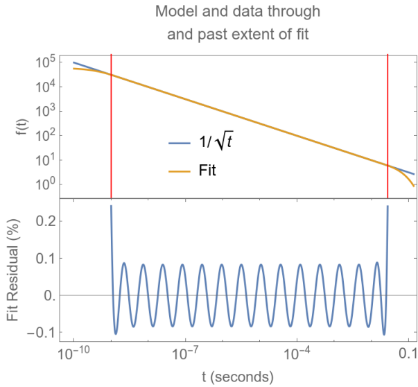
Figure 2: Fit of pseudomodes to the 1/\sqrt{t} dependence of the long-range resistive wall wake. The vertical red bars indicate the fitted region, which extends from 1 ns to 26.7 ms (equivalently said: one-half of a 500 MHz bucket to 44000 turns). Within the fitted region, the fit is good to 0.1%. Outside the region, the fit reliably decays to zero.
