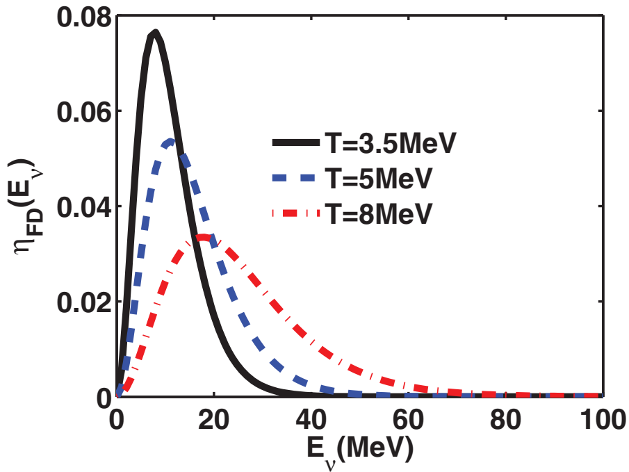
Figure 2. The normalized unity Fermi-Dirac spectrum for \alpha = 0 .
