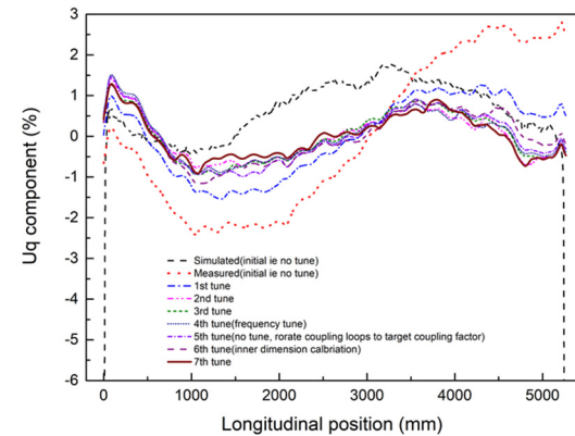
Figure 2: Evolution of the quadrupole perturbative component during tuning.
