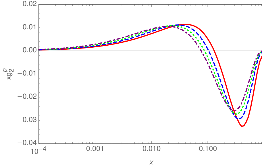
Figure 2: The NLO massless structure function g_2(x, Q^2) as a function of x for Q^2 = 10 \text{ GeV}^2 (full line); 100 \text{ GeV}^2 (dashed line); 1000 \text{ GeV}^2 (dotted line), and 10000 \text{ GeV}^2 (dash-dotted line), [26].
