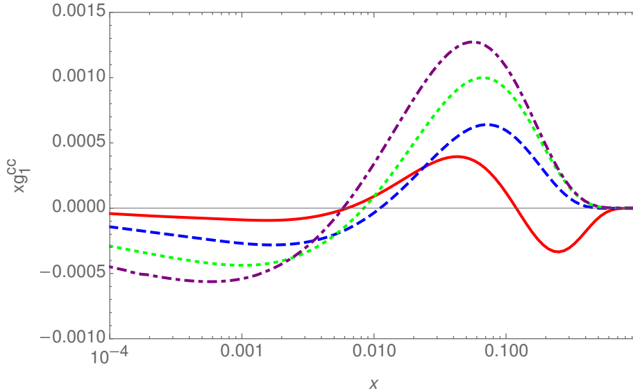
Figure 3: The O(a_s) charm contribution the polarized structure function g_1(x, Q^2) as a function of x for Q^2 = 10 \text{ GeV}^2 (full line); 100 \text{ GeV}^2 (dashed line); 1000 \text{ GeV}^2 (dotted line), and 10000 \text{ GeV}^2 (dash-dotted line) for m_c = 1.59 \text{ GeV} and the parton distribution functions [26].
