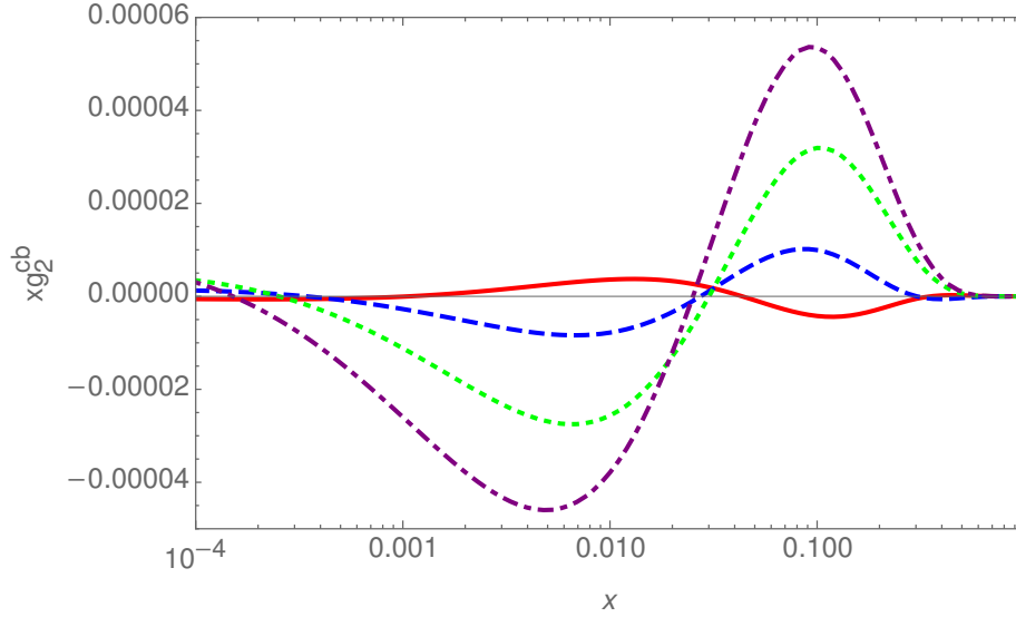
Figure 12: The O(a_s^2) two-mass contribution the polarized structure function g_2(x, Q^2) as a function of x for Q^2 = 10 \text{ GeV}^2 (full line); 100 \text{ GeV}^2 (dashed line); 1000 \text{ GeV}^2 (dotted line), and 10000 \text{ GeV}^2 (dash-dotted line) for m_c = 1.59 \text{ GeV} and m_b = 4.78 \text{ GeV} and the parton distribution functions [26].
