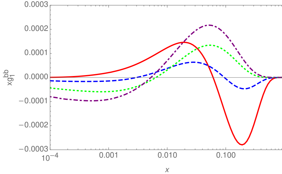
Figure 5: The O(a_s) bottom contribution the polarized structure function g_1(x, Q^2) as a function of x for Q^2 = 10 \text{ GeV}^2 (full line); 100 \text{ GeV}^2 (dashed line); 1000 \text{ GeV}^2 (dotted line), and 10000 \text{ GeV}^2 (dash-dotted line) for m_b = 4.78 \text{ GeV} and the parton distribution functions [26].
