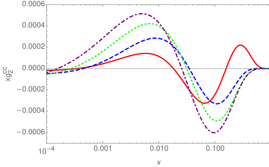
Figure 4: The O(a_s) charm contribution the polarized structure function g_2(x, Q^2) as a function of x for Q^2 = 10 \text{ GeV}^2 (full line); 100 \text{ GeV}^2 (dashed line); 1000 \text{ GeV}^2 (dotted line), and 10000 \text{ GeV}^2 (dash-dotted line) for m_c = 1.59 \text{ GeV} and the parton distribution functions [26].
