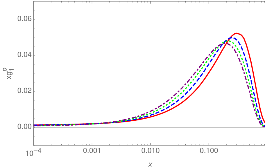
Figure 1: The NLO massless structure function g_1(x, Q^2) as a function of x for Q^2 = 10 \text{ GeV}^2 (full line); 100 \text{ GeV}^2 (dashed line); 1000 \text{ GeV}^2 (dotted line), and 10000 \text{ GeV}^2 (dash-dotted line), [26].
