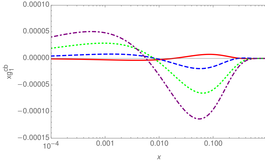
Figure 11: The O(a_s^2) two-mass contribution the polarized structure function g_1(x, Q^2) as a function of x for Q^2 = 10 GeV 2 (full line); 100 GeV 2 (dashed line); 1000 GeV 2 (dotted line), and 10000 GeV 2 (dash-dotted line) for m_c = 1.59 GeV and m_b = 4.78 GeV and the parton distribution functions [26].
