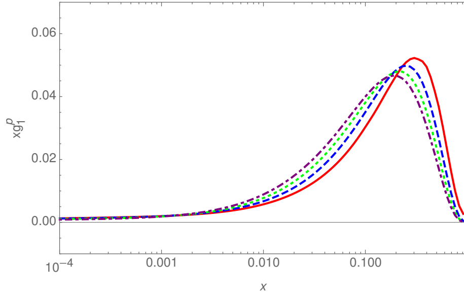
Figure 8: The O(a_s^2) massive contributions to the structure function g_1^{bb}(x, Q^2) for m_c = 4.78 GeV as a function of x for Q^2 = 10 GeV ^2 (full line); 100 GeV ^2 (dashed line); 1000 GeV ^2 (dotted line), and 10000 GeV ^2 (dash-dotted line), [26].to be done
