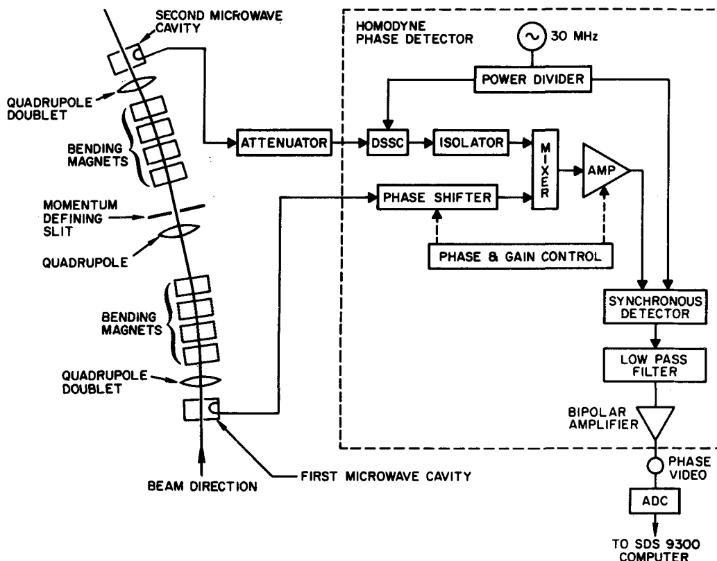
Fig. 1. Precision energy measurement system.
