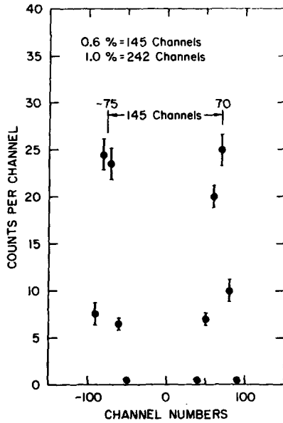
Fig. 2. Calibration of energy monitor by energy wobbling.
