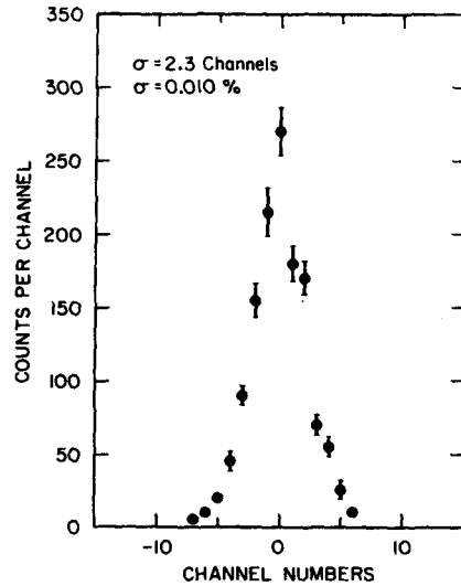
Fig. 3. Pulse-to-pulse energy jitter during stable run.
