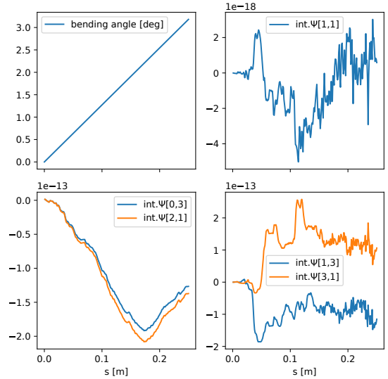
Figure 2: Cumulative integral of polynomial coefficients of homogenic vertical field. The curves \text{int.}\Psi[p, q] hold the coefficients \Psi_{j pq} cumulatively integrated in s_j using trapezoid rule. From top left to bottom right: bending angle, quadrupole coefficient, (both upright) sextupole polynomial coefficients, octupole coefficients.
