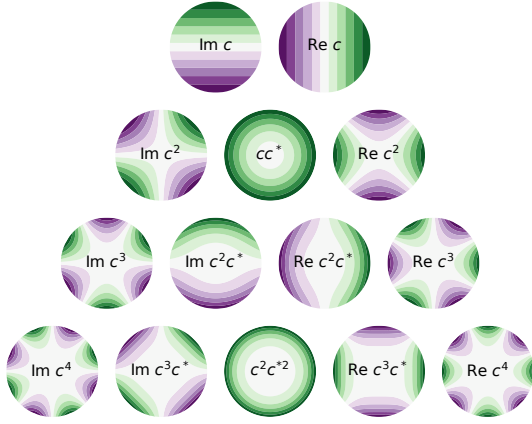
Figure 1: Alternative 2d basis functions for \tilde{\Omega} using a complex number c = x + iy , inspired by [6] and Zernike polynomials. Left and right edges of the triangle show standard upright and skew multipoles, which have no in-plane divergence. The interior maps fringe-like effects. In magnets with machine-plane symmetry, only “Im” entries occur.
