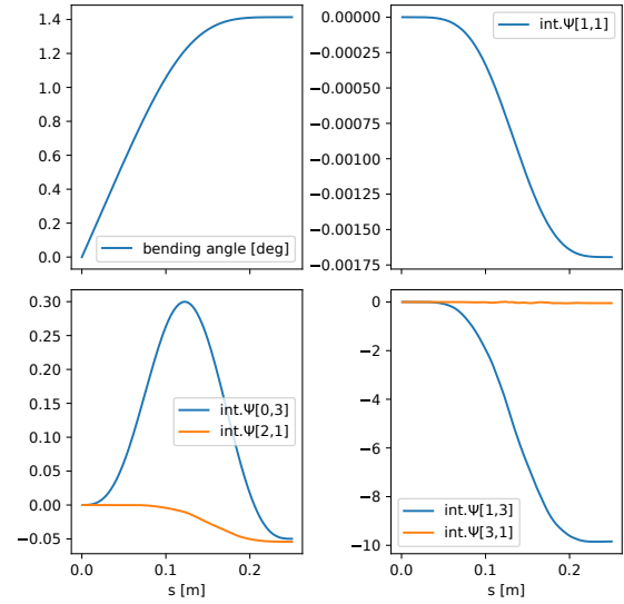
Figure 5: Cumulative integral of polynomial coefficients of dipole with edge. See Fig. 2 for legend.
