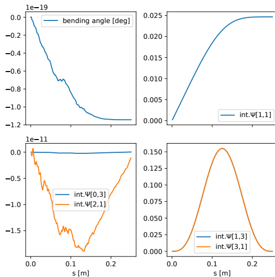
Figure 4: Cumulative integral of polynomial coefficients of quadrupole with edge. See Fig. 2 for legend.
