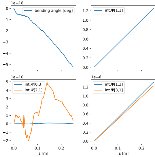
Figure 3: Cumulative integral of polynomial coefficients of homogenic quadrupole. See Fig. 2 for legend.
