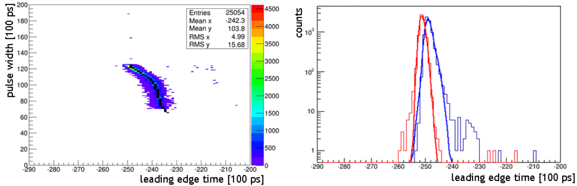
Figure 2. TOT plot (left) and time distributions in logarithmic scale before (blue) and after (red) time walk correction (right).
