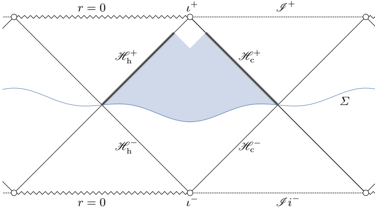
Fig. 1. Construction of the counterexample.
