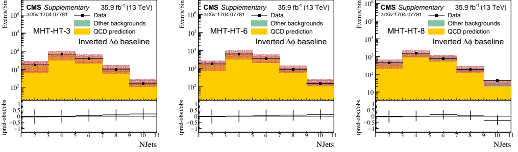
Figure 5. Comparison between the predicted and observed jet multiplicity distributions in the low \Delta\phi control region in numbered kinematic regions defined in Fig. 2. The rebalance and smear QCD prediction is shown in yellow and the other backgrounds, determined by methods described herein, are in green. The red uncertainty band indicates the statistical and systematic uncertainties in the background prediction summed in quadrature.
