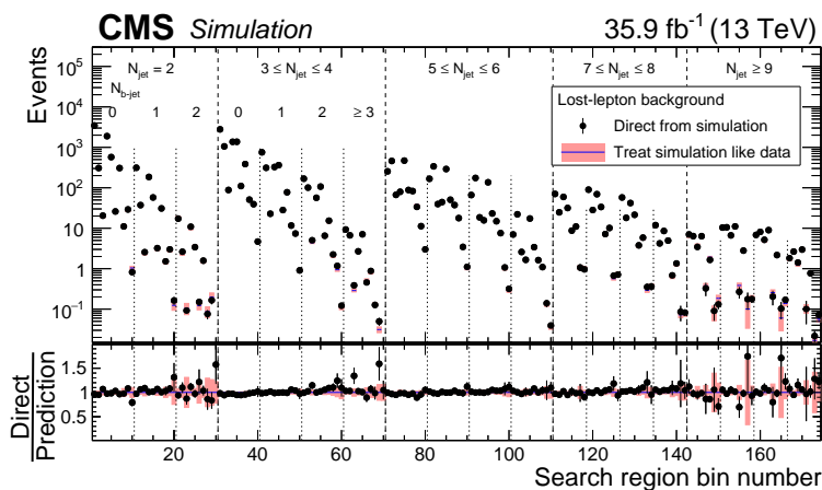
Figure 3. The result of the lost lepton background prediction method applied to simulated even samples compared with the counts obtained directly from simulation, as published in [2]. Uncertainties shown are statistical.
