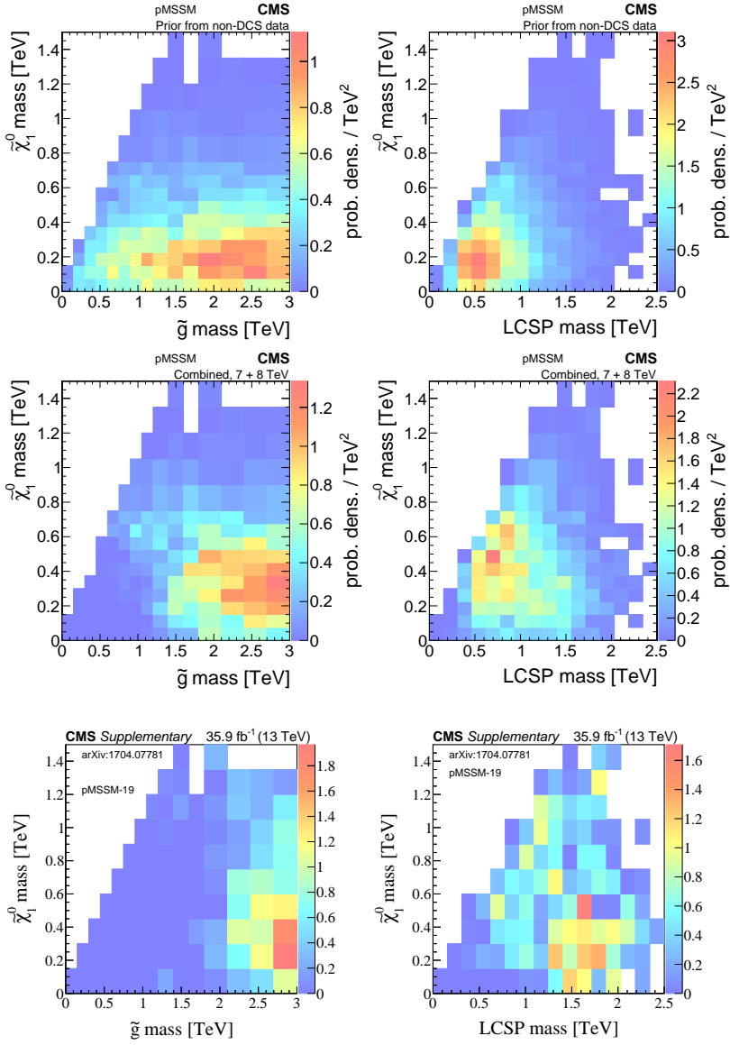
Figure 9. The pMSSM probability density corresponding to the prior (top) before any CMS constraints have been applied, the posterior density after the constraints of the 7 and 8 TeV SUSY searches have been incorporated as published in [8] (center), and the posterior density after all analyses including the 13 TeV multi-jet search have been incorporated.
