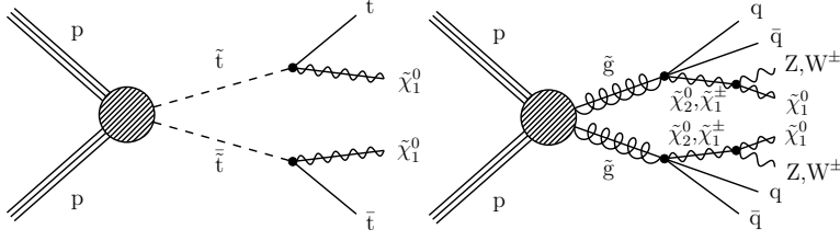
Figure 1. Two of several simplified model diagrams motivating the search strategy.
