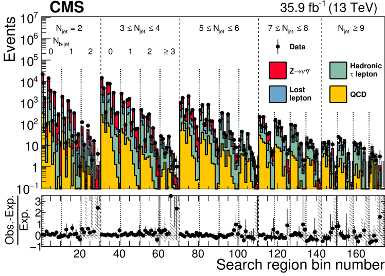
Figure 6. The observed count in each signal region, compared with the sum of the predictions for the various background contributions, as published in [2].
