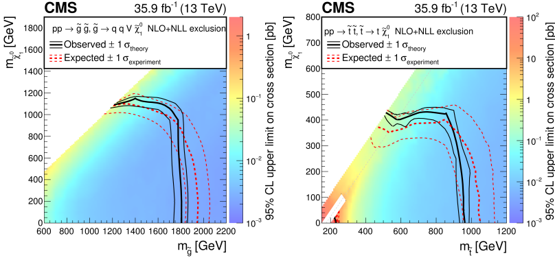
Figure 7. The color map gives the 95% CL upper limit on the cross section as calculated by the CLs procedure. Black (red) lines indicate the upper limit assuming the nominal cross section. Figures as published in [2].
