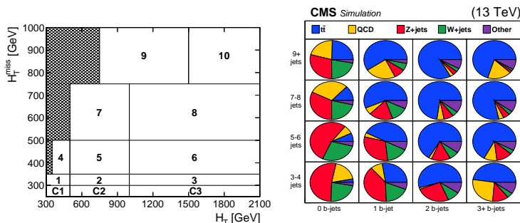
Figure 2. Left: boundaries of the signal regions (numbered) and control regions (C1, C2, C3) in the H_T – H_T^{\text{miss}} plane. Right: boundaries of the signal regions in the plane of n_{\text{jet}} and n_b , with the relative contribution to background events from the four primary sources, integrating over all H_T and H_T^{\text{miss}} . n_{\text{jet}} = 2 bins are not shown.
