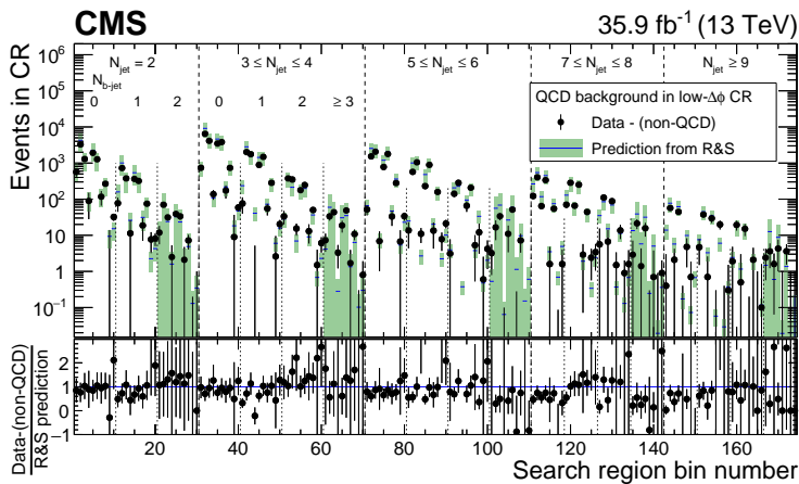
Figure 4. The result of the rebalance and smear prediction method applied to real events and evaluated in each inverted \Delta\phi control region bin, compared with the observed count less the predicted non-QCD count, as published in [2]. Uncertainties shown are statistical and systematic.
