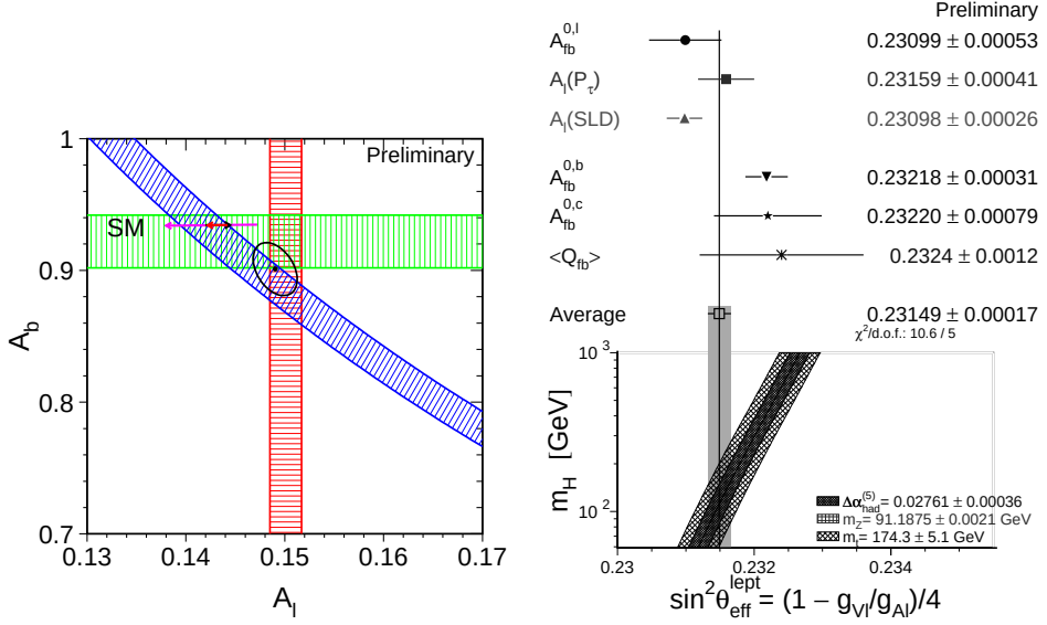
Fig. 1. (Left): The measurements of the combined LEP+SLD A_l = 0.1501 \pm 0.0016 (vertical band), SLD A_b (horizontal band) and LEP A_{FB}^{0,b} (diagonal band), compared to the SM expectations (arrow). Also shown is the 68 % CL contour for the two asymmetry parameters resulting from the joint analysis. (Right): Comparison of several determinations of \sin^2 \theta_{\text{eff}}^{\text{lept}} from A_{FB}^{0,l} , A_l(P_\tau) , A_l(\text{SLD}) , A_{FB}^{0,b} , A_{FB}^{0,c} and \langle Q_{FB} \rangle measurements. Also shown is the SM prediction as a function of m_H . The width of the Standard Model band is due to the uncertainties in \Delta\alpha_{\text{had}}^{(5)}(m_Z^2) , \Delta\alpha_s(m_Z^2) and m_t .
