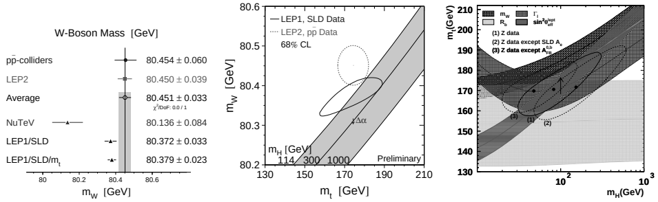
Fig. 2. (Left): The world average of the direct m_W measurements from p\bar{p} colliders and LEP2. Also shown are the indirect m_W measurements by NuTeV, LEP1+SLD and LEP1+SLD with m_t measurements.
