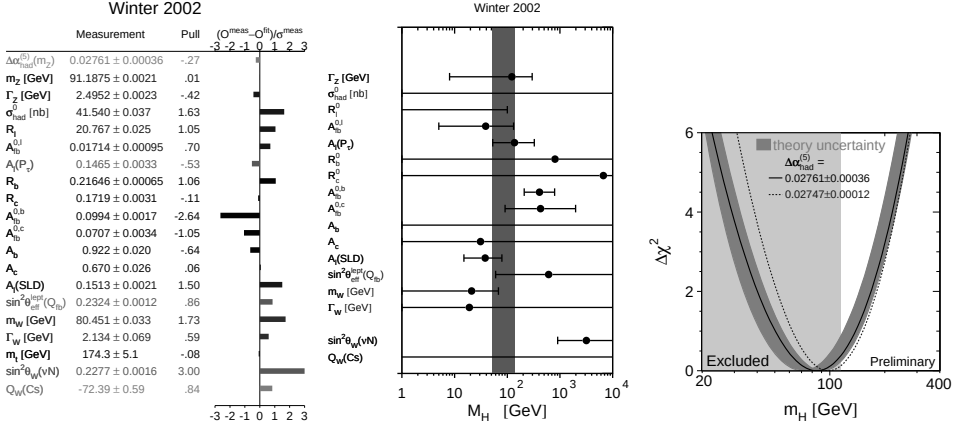
Fig. 3. (Left): The pulls (difference between measurement and fit in units of the total measurement error) of the SM fit including all data.
