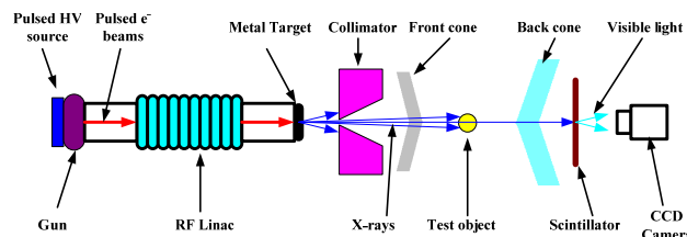
Figure 1: Layout of a typical flash X-ray radiography system using RF accelerator.
