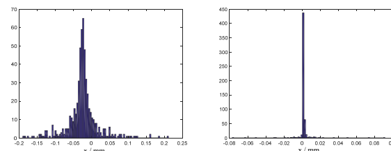
Figure 8: Horizontal distribution of beam obits dispersion at the exit with shot width of accelerator structures as 1 mm (left) and 3 mm (right).
