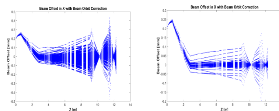
Figure 7: Simulation results of horizontal beam obits dispersion along the accelerating axis with a 200ns RF duration (including RF fill-up time) considering long-range wakefield with shot width of accelerator structures as 1 mm (left) and 3 mm (right).
