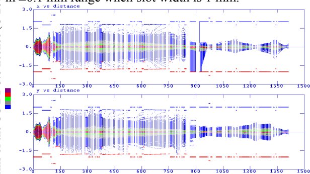
Figure 5: Beam envelope calculation result.
