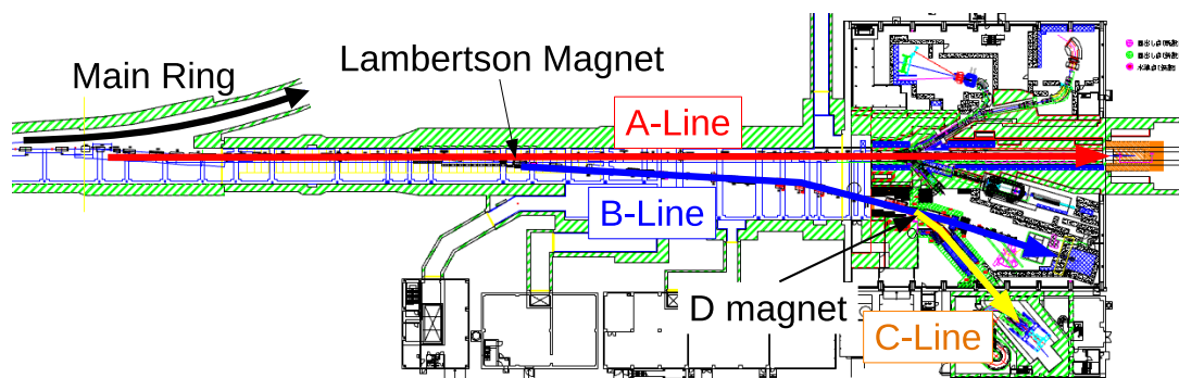
Figure 2: Proton beamlines at the Hadron Facility.
