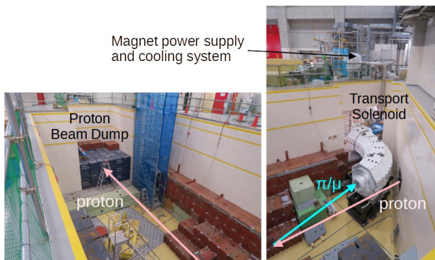
Figure 4: The COMET primary target room.
