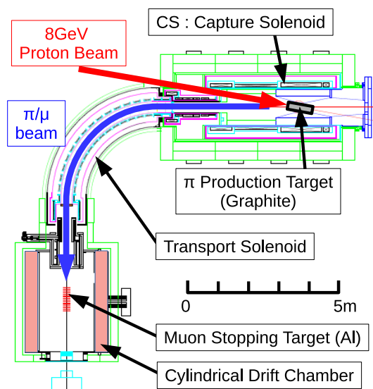
Figure 1: The COMET experiment setup at Phase-1.
