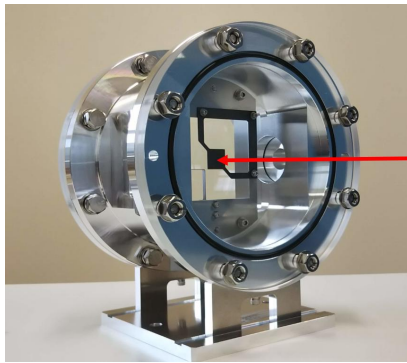
Figure 6: Target chamber for the COMET phase- \alpha . The arrow indicates the proton beam direction.
