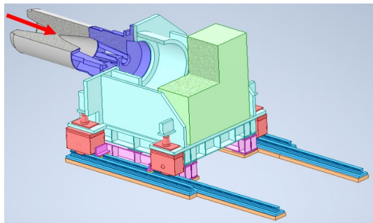
Figure 7: Inner shield of the Capture Solenoid and its carriage platform. The arrow indicates the proton beam direction. The target will be positioned at the tip of the arrow.
