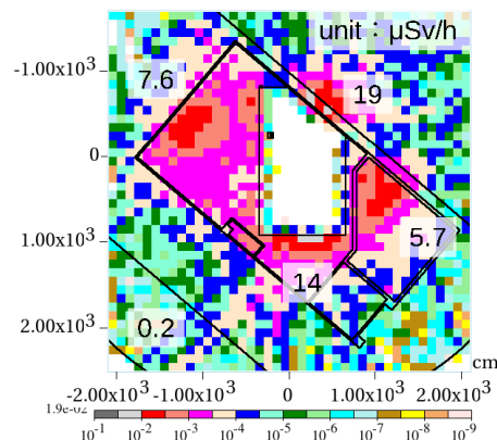
Figure 8: Prompt dose of the first floor of the experimental hall during beam operation.
