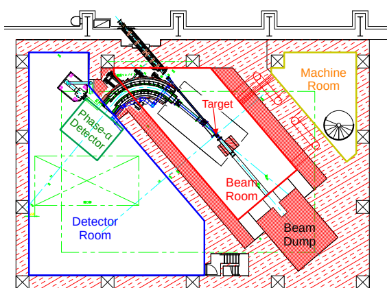
Figure 3: Plan view at the beam level.
