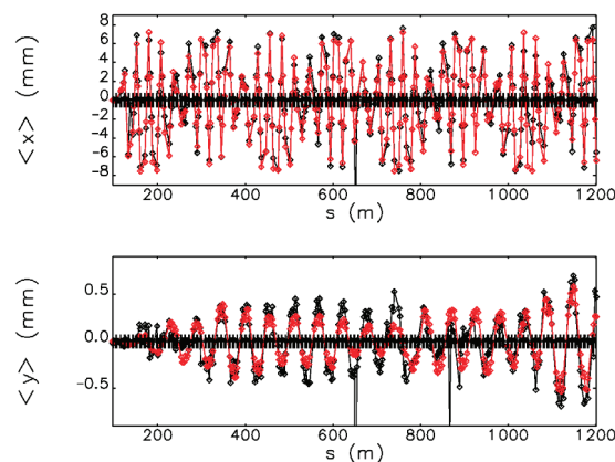
Figure 3: IK1 3-kV calibration: BPM data (black) compared with elegant 0.33 mrad kick (red).
