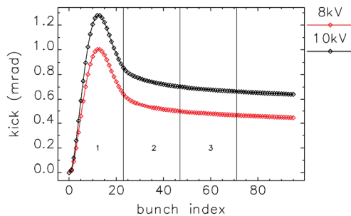
Figure 1: Abort kicker waveform kick angles calculated from measured integrated field B \cdot dl divided by B_p . The first three turns are marked.
