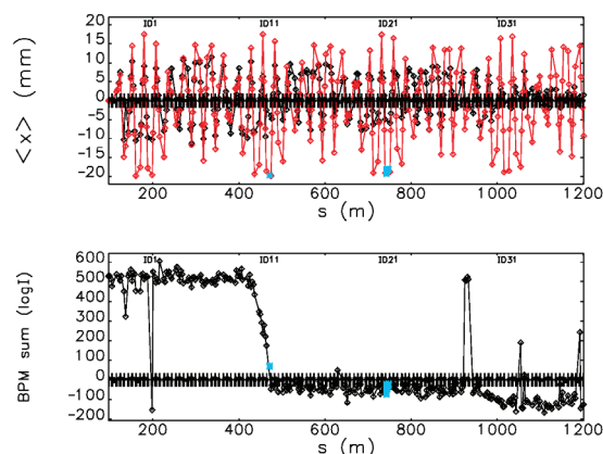
Figure 4: Trajectory (top) and loss distribution (sum, bottom) with IK1 at 7.5 kV, compared with elegant 0.8 mrad (red) and simulated loss distribution (cyan).
