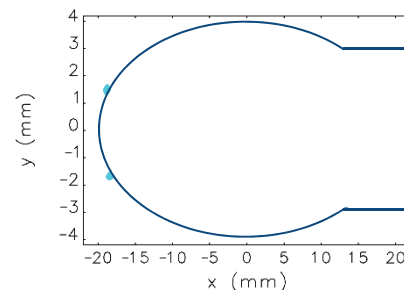
Figure 2: Simulated beam losses (cyan) on ID19 chamber shown with schematic of chamber profile.
