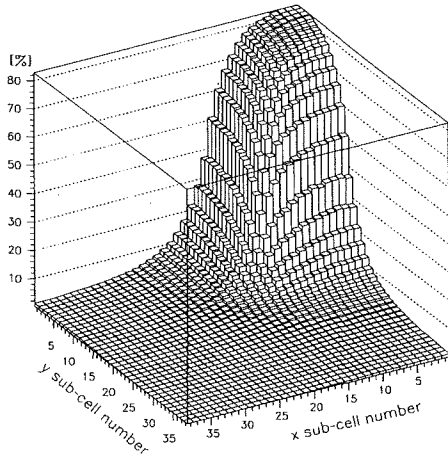
Fig. 12. The lego plot of the shower table.
