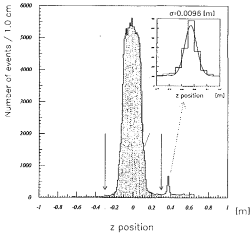
Fig. 15. The distribution of z positions of event vertices reconstructed from the data of MWPC's. The events with the z vertex within \pm 0.3 m from the target center have been selected. At 0.37 m downstream the target, the peak came from the aluminum plate of 2 mm thick.
