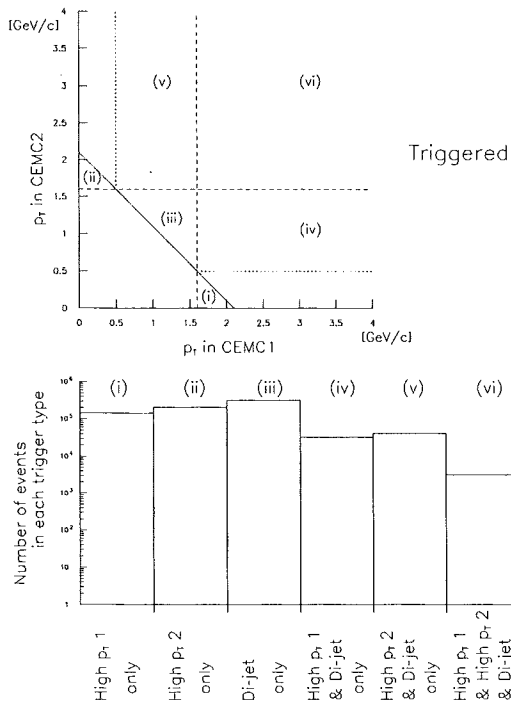
Fig. 9. The relation among the “high p_T trigger” for CEMC1, the “high p_T trigger” for CEMC2 and the “di-jet trigger”. The trigger rates for each region are shown in the histogram exclusively.
