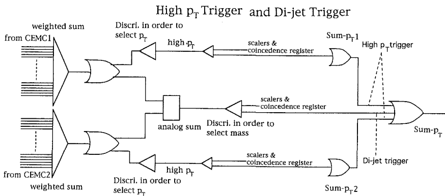
Fig. 8. Scheme of the “high p_T trigger” and the “di-jet trigger”.
