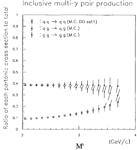
Fig. 28. The contributions of gluon-gluon, gluon-quark and quark-quark scatterings to the inclusive multi- \gamma pair production obtained from the Monte-Carlo simulation with the Duke-Owens set 1. The error bars indicate the statistical errors.
