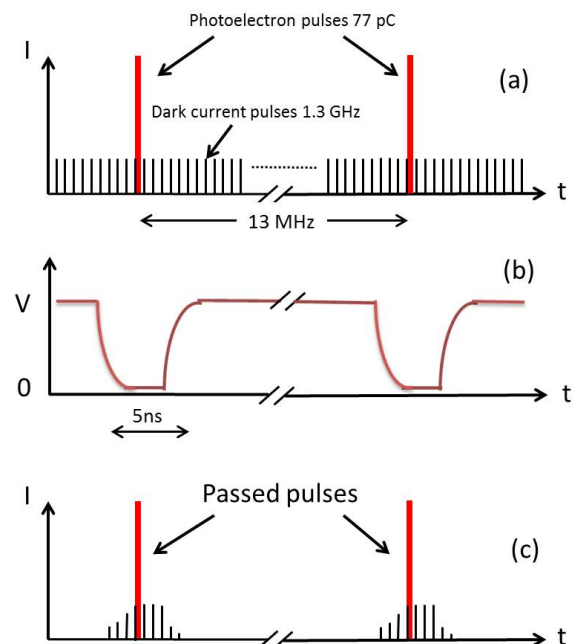
Figure 7: The concept of the kicker designed for SRF gun.
