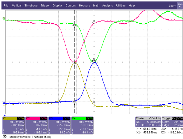
Figure 4: Output pulse of all 4 channels measured after the termination attenuators.
