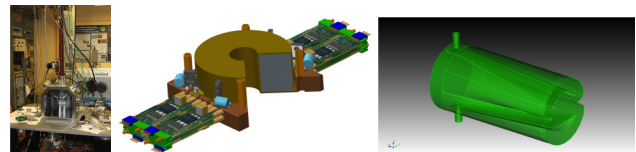
Figure 6: Left: Coating test setup for small NEG chambers. Middle: Single stage of inductive adder for fast injection magnets. Right: Tapered end of small aperture stripline kicker.
