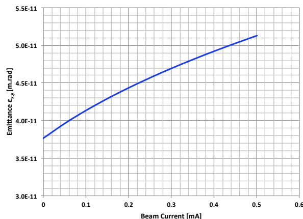
Figure 3: Predicted increase in emittance due to intra beam scattering including the effects of a typical full set of insertion devices, assuming a bunch lengthening factor of four by using a third harmonic cavity system.
