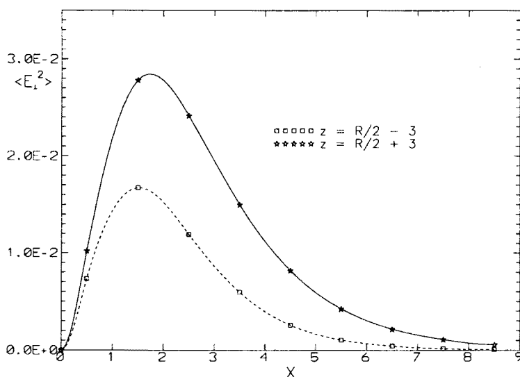
Fig. 16. Transverse dependence for \langle E_{\perp}^2 \rangle and two different z .
