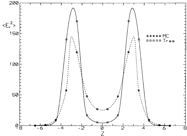
Fig. 18. Perturbative vs. Monte Carlo data: longitudinal profile for \langle E_{||}^2 \rangle .
