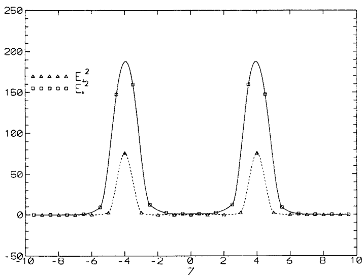
Fig. 15. Longitudinal profiles for \langle E_{\parallel}^2 \rangle and \langle E_{\perp}^2 \rangle .
