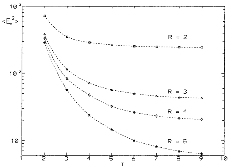
Fig. 19. \langle E_{||}^2 \rangle at the mid-point between the quarks as a function of temporal extent of the Wilson loop.
