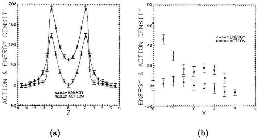
Fig. 5. Energy and action density for the loop 4 \times 4 — interpolated longitudinal and transverse profiles
