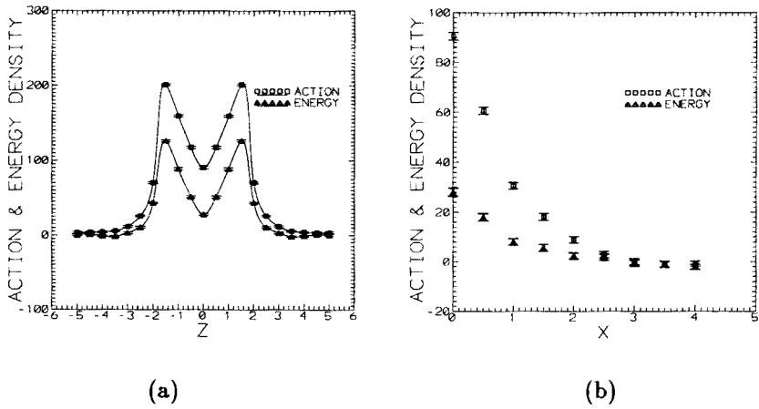
Fig. 4. Energy and action density for the loop 3 \times 3 — interpolated longitudinal and transverse profiles
