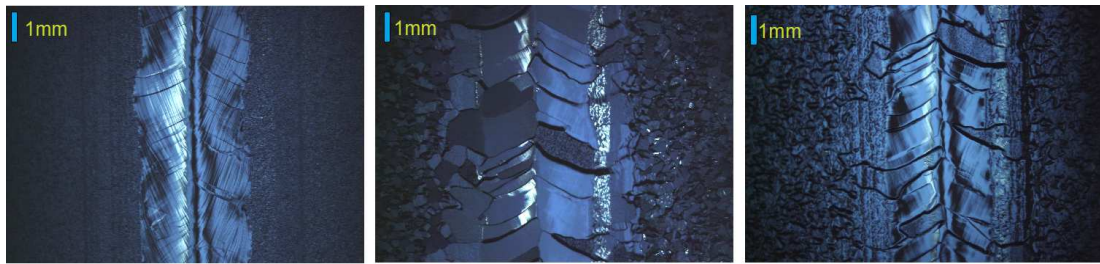
Figure 3: Equatorial welding seam of cell 1 in Z137: before EP (left), after main-EP (center) and after final-EP (right)
