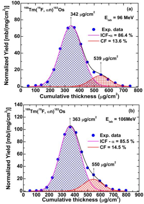
Fig.1 (a-b) Experimentally measured recoil range distribution of ^{183}\text{Os} residues populated through \alpha n channel in ^{19}\text{F} + ^{169}\text{Tm} system at two incident energies 96 and 106 MeV.
