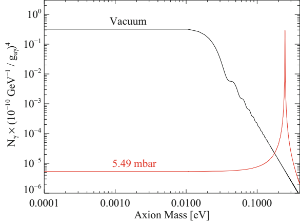
Fig. 5.7 Expected number of photons from axion-to-photon conversion in a magnetic field for a typical axion helioscope as described in the text (namely, CAST). The pressure of the buffer gas (here, ^4\text{He} ) is given at 1.8 K and therefore 5.49 mbar corresponds to a density of 0.147 \text{ kg/m}^3
