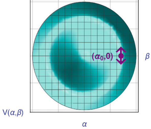
Fig. 2.4 Overhead view of the potential V(\alpha, \beta) from Eq. (2.22). The purple dot indicates the (arbitrary) ground state after spontaneous symmetry breaking at (\alpha = \alpha_0 = \sqrt{6\mu^2/\lambda}, \beta = \beta_0 = 0) . The double-headed purple arrow indicates small perturbations of the \beta field around \beta = \tilde{\beta} = 0 , requiring approximately zero energy as seen from Eq. (2.32). Thus the quantum excitations of the \beta field are massless bosons, a consequence of Goldstone’s theorem
