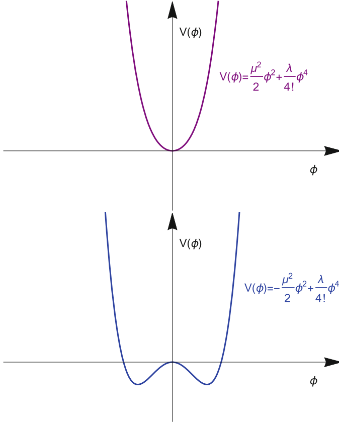
Fig. 2.2 The purple plot on the top shows a quartic scalar field potential V(\phi) with a positive quadratic term [Eq. (2.20)], the blue plot on the bottom shows V(\phi) with a negative quadratic term [Eq. (2.21)]
