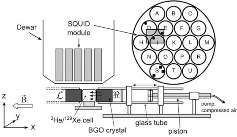
Fig. 8.5 Schematic diagram of the experimental setup from Ref. [45] used to search for anomalous monopole-dipole interactions. The ^3\text{He}/^{129}\text{Xe} cell is located at the center. The BGO crystal is placed on right (or left) side with respect to the sample. The crystal travels back and forth toward the cell with a certain frequency. The SQUID module located on the top of the cell monitors the precession frequency of each species. Adapted from Ref. [45]
