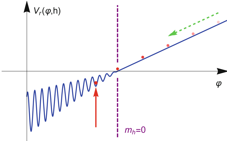
Fig. 2.8 Plot of the relaxion potential V_r(\varphi, h) and illustration of the dynamics. The relaxion field \varphi starts at a relatively large value (shown by the faded red dots) and then “slowly rolls” down the potential (as indicated by the green dashed arrow), decreasing in amplitude, which in turn decreases m_h according to Eq. (2.125). When the Higgs’ vacuum expectation value becomes nonzero at the onset of spontaneous symmetry breaking at m_h = 0 (marked by the dashed purple line), the amplitude of the periodic potential for \varphi increases. Shortly after spontaneous symmetry breaking occurs the potential wells become too deep and \varphi becomes trapped in a local minimum (shown by the leftmost red dot marked by the red arrow), which sets the scale of m_h at a value \ll \Lambda , far from the Planck scale
