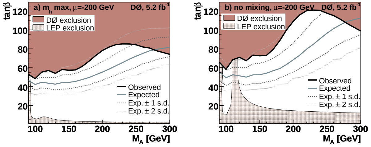
FIG. 6: (color online) a) 95% C.L. lower limit in the (M_A, \tan\beta) plane obtained for the m_h^{\max}, \mu = -200 GeV scenario, b) the lower limit for the no-mixing, \mu = -200 GeV scenario. The one and two standard deviation bands around the expected limit and the exclusion limit obtained from the LEP experiments are also shown [4].
