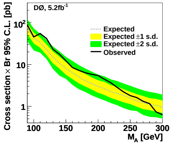
FIG. 5: (color online) Model independent 95% C.L. upper limit on the cross section multiplied by the branching ratio for the combined 5.2 \text{ fb}^{-1} analysis. The light and dark grey regions correspond to the one and two standard deviation (s.d.) bands around the expected limit.
