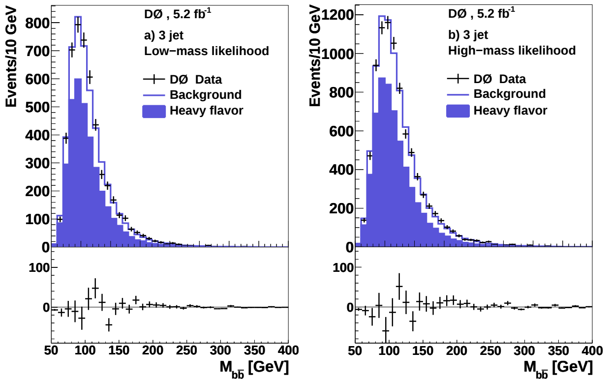
FIG. 2: (color online) Invariant mass distribution for the 3Tag exclusive three-jet channel for: a) the low-mass likelihood selection and b) the high-mass likelihood selection. Each event has one entry, the jet pairing with the highest likelihood output. Black crosses refer to data, the solid line shows the total background estimate, and the shaded region represents the heavy flavor component ( b\bar{b}b , b\bar{b}c , and bc\bar{c} ). The lower panels show the difference between the data and the predicted background.
