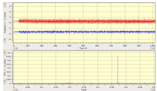
Figure 8: Transverse turn-by-turn beam position and betatron tune measurements using new calibrated BPM in the DR.
