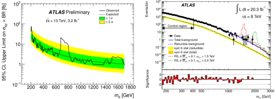
Fig. 11. Left: Expected and observed upper limits on \sigma_{fid} \times BR(X \rightarrow \gamma\gamma) expressed at 95% C.L., as a function of the assumed value of the narrow-width scalar resonance mass m_X . Taken from [39]. Right: Observed di-photon invariant mass distribution with superimposed the SM background prediction. The bin-by-bin significance of the difference between data and background expectation is shown in the bottom panel. Taken from [40].
