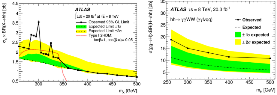
Fig. 8. The observed and expected upper limit at 95% C.L. on the \sigma(gg \rightarrow X) \times \text{BR}(X \rightarrow hh) as a function of m_X from the resonant \gamma\gamma bb analysis (left) and on \sigma(gg \rightarrow H) \times \text{BR}(H \rightarrow hh) as a function of m_H from the resonant hh \rightarrow \gamma\gamma WW^* analyses (right). Taken from [34, 36].
