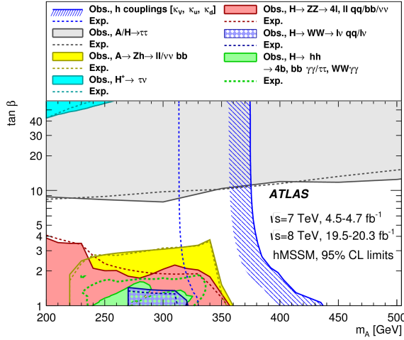
Fig. 2. Regions of the [m_A, \tan\beta] plane excluded in the hMSSM model via fits to the measured rates of Higgs boson production and decays. The likelihood contours where -2 \ln \Lambda = 6.0 , corresponding approximately to the 95% C.L. (2 std. dev.), are indicated for the data and expectation for the SM Higgs sector. Taken from [18].
