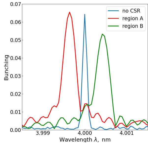
Figure 5: The bunching spectrum around the target wavelength. For regions A and B the bunching is normalized to the number of particles inside the corresponding region.
