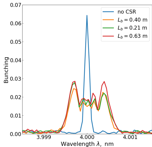
Figure 3: The bunching spectrum around the target wavelength.
