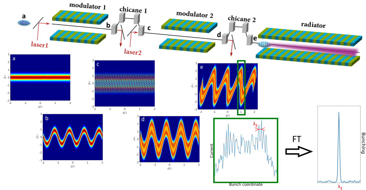
Figure 1: The electron bunch travels through 2 modulators and 2 chicanes before the radiator (top), the heat map plots of the longitudinal phase space of the electron bunch at positions a-e (middle), the current profile of a bunch slice and its Fourier transform around the target wavelength \lambda_t (bottom-right).
