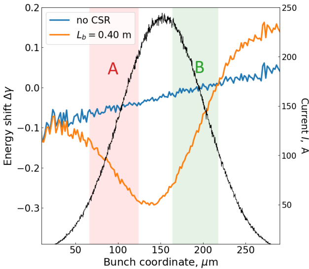
Figure 4: The energy profile of the electron bunch with CSR disabled (blue), the CSR-induced energy modulation for L_b = 0.4 m with two selected regions and the current profile (black) along the bunch after chicane 1. The energy shift is calculated with respect to the nominal beam energy.
