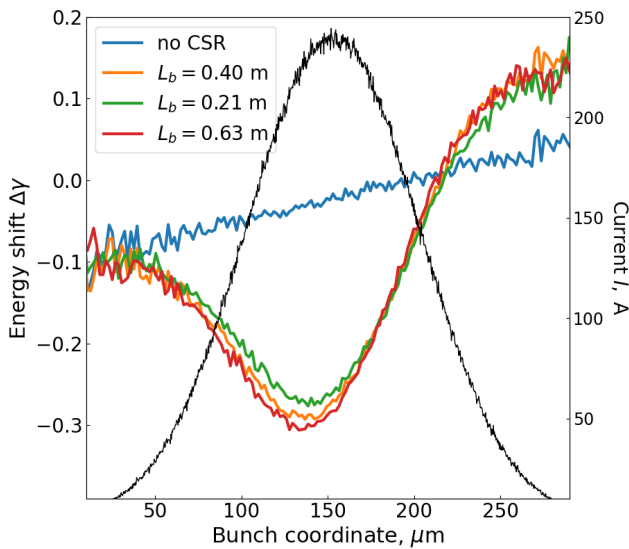
Figure 2: The energy profile of the electron bunch with CSR disabled (blue), the CSR-induced energy modulation for different dipole lengths and the current profile (black) along the bunch after chicane 1. The energy shift is calculated with respect to the nominal beam energy.
