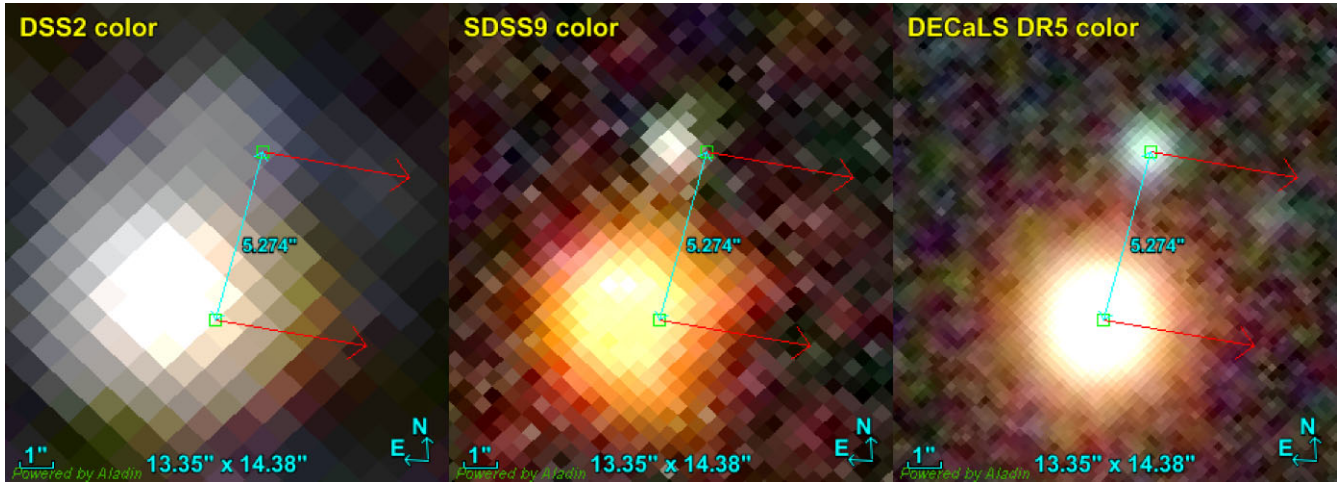
Figure C1. Sequence of DSS2- (1995–1996), SDSS- (2005), and DECaLS (2015–2017-epoch) colour images showing that P18 is comoving with the brighter and redder star, Gaia DR3 3948582104883968384. The small green squares indicate the Gaia DR3 positions at epoch 2016.0, and the red arrows indicate the proper motions, magnified to show their equality.
