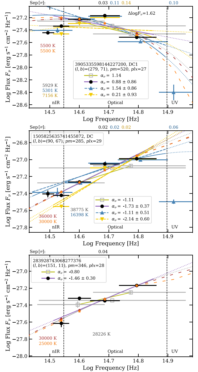
Figure B1. SEDs of three white-dwarf sources with griz -band flux profiles that are: (top panel) very curved (‘DC1’), (middle panel) curved-up (large \alpha_\nu , peaking at gr bands, and with significantly suppressed u -band flux (Gaia DR3 1505825635741455872), (bottom panel) straight-up with an apparent i -band flux excess (Gaia DR3 283928743068277376). Same as in Fig. 10.
