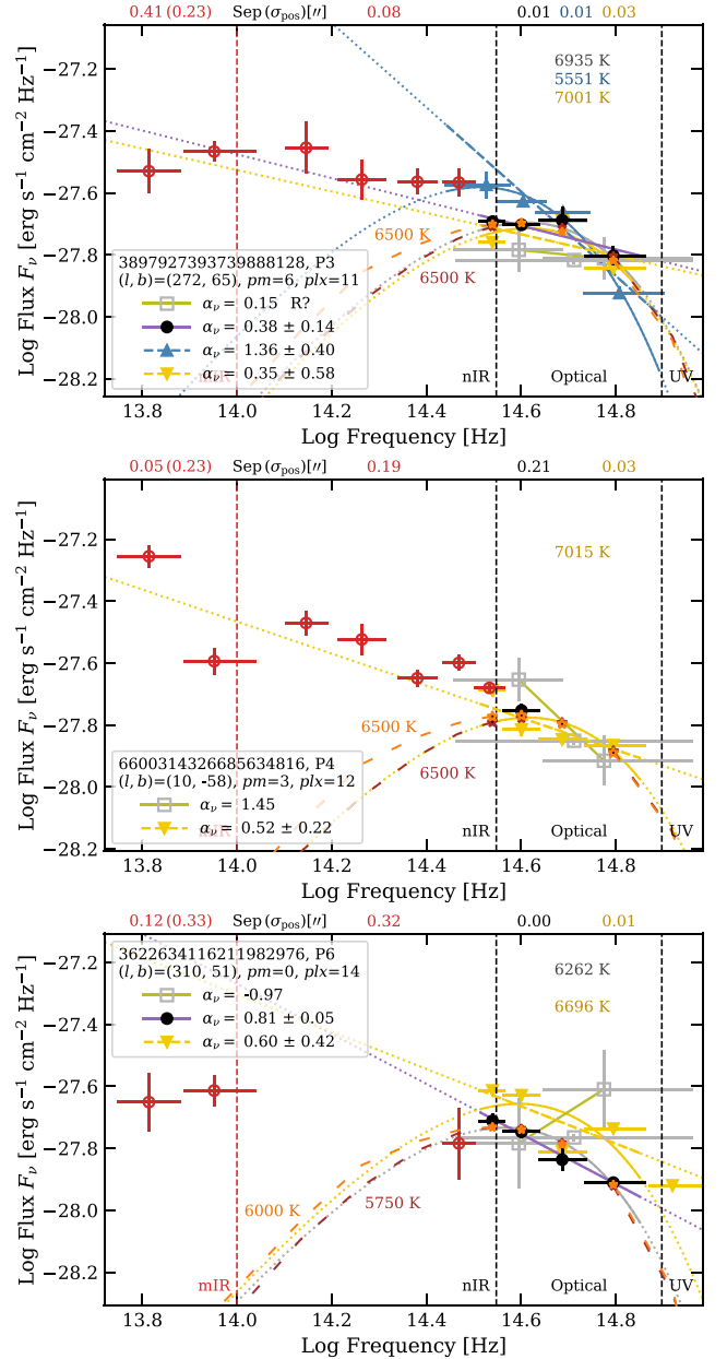
Figure 15. SEDs of P3, P4, and P6, which have approximately straight infrared–optical profiles (UV7 is shown in Fig. 18). Same as in Fig. 10.
