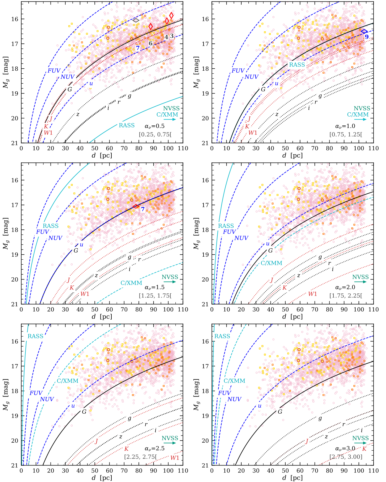
Figure 7. Same as Fig. 6, for power-law emitters of spectral index \alpha_\nu = 0.5, 1, 1.5, 2, 2.5, and 3 .
