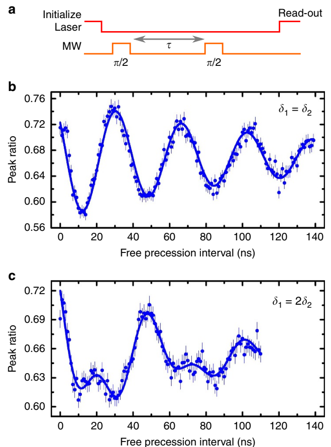
Figure 4 | Ramsey interferometry. (a) Microwave and optical pulses protocol: two microwave \pi/2 pulses of 8 ns each are separated by a variable delay \tau . The time interval between the initialization and read-out pulses is held constant at 160 ns, not to include the effect of the spin population decay into the signal. (b) Variation of the peak ratio as a function of the delay between the microwave pulses (blue dots) at 3.6 K (error bars correspond to the s.d. of the peak ratio). The microwave frequency is fixed at the average of the two resonance frequencies (the detuning \delta_1 from the lower frequency transition equals the detuning \delta_2 from the other). The blue solid curve is a fit of the form \cos(2\pi \cdot \tau \cdot \delta) \exp(-\tau/T_2^*) , where \delta is the common detuning between the microwave frequency and the two resonances. We extract T_2^* = 115 \pm 9 ns (the error corresponds to the s.d. on the fit parameter). (c) The duration of the microwave pulses is kept unchanged compared to b, but the frequency is tuned such that the detuning from one resonance is twice that with the other ( \delta_1 = 36 MHz and \delta_2 = 18 MHz). The solid curve is a fit where the cosine function in b is replaced by the sum of two cosine functions, with frequencies corresponding to the respective detunings.
