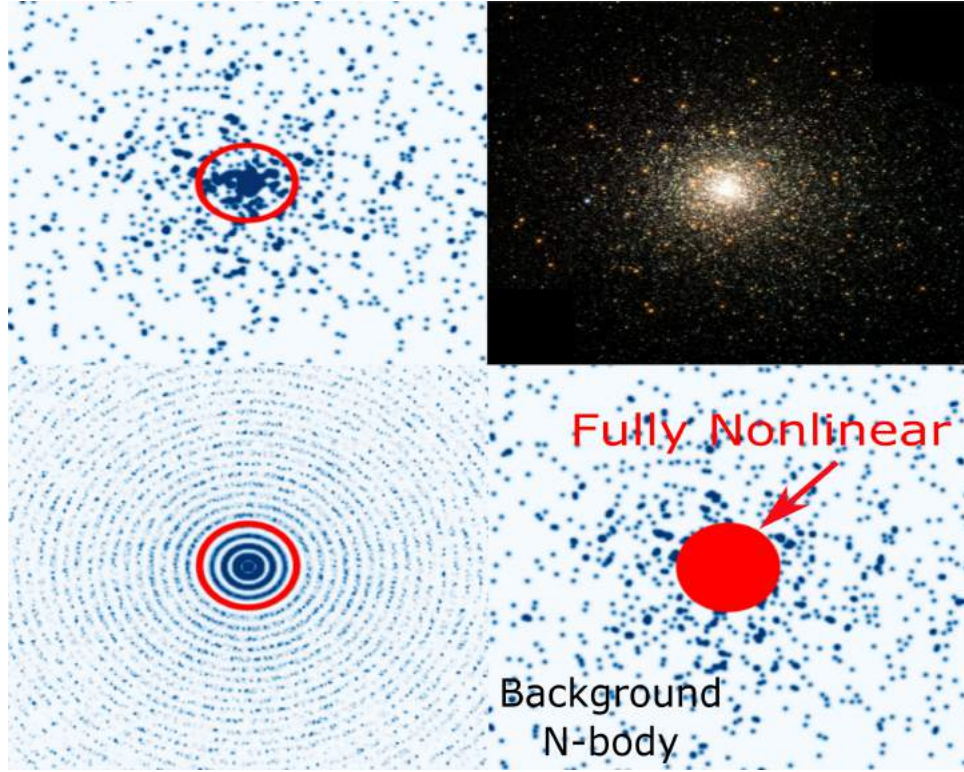
FIGURE 3.6: Background Boundary Conditions: A motivation for \text{SF}\psi\text{DM} boundary conditions. Top left: A system of DM particles placed to emulate an N-body system; particles are uniformly distributed by radius, and randomly distributed by angle. Saturation effects are applied for visualization. Top right: A globular cluster demonstrating a real N-body system. Bottom left: The same as the top left image, but distributed uniformly in angle to compare to a spherically symmetric setting. Bottom right: A possible description of \text{SF}\psi\text{DM} halos. As seen in the top left image, the particles become densely packed in the central regions of the halo resulting in a large amount of interference and overlap. In the bottom left image, we can identify the radius at which the particles begin to display substantial overlap, this is shown with a red circle. Outside of this boundary the particles can be individually resolved while inside the boundary they cannot. The bottom right image suggests describing the central region as a fully nonlinear solution to the EKGEs, characterized by the overlap of the halo's many DM particles. The outer region of the halo can then be thought of as an N-body problem of DM particles evolving in the gravitational well of the halo.
