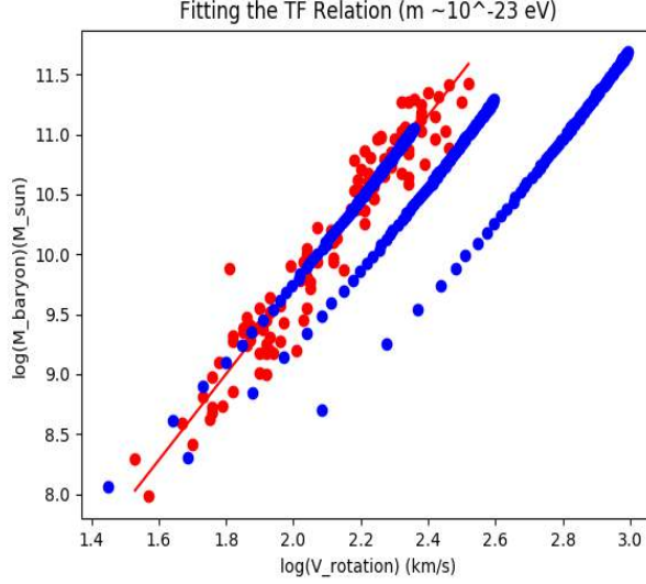
FIGURE 3.9: Fitting the BTFR via Boundary Conditions: An example of the fitting routine for the BTFR using m = 10^{-23}\text{eV} . First, the boundary problem is imposed on sequence of excited states, resulting in a BTFR-like relation. Next, the boundary values are adjusted until the simulated relation overlaps the data (shown as the progression of the 3 simulations in blue). Scaling the boundary values shifts the entire relation, maintaining its slope. The relation extends indefinitely towards higher masses, but the minimum mass is bounded from below by the ground state profile.
