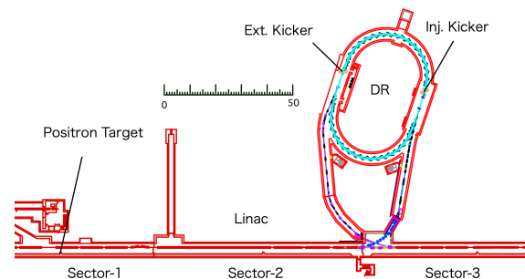
Figure 1: Schematic layout of Linac and DR for SuperKEKB.
