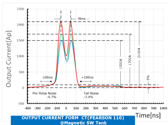
Figure 5: Output current of the kicker magnet without the ceramic duct.
