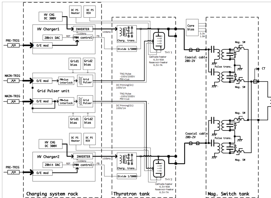
Figure 2: Block diagram of the DR kicker power supply.
