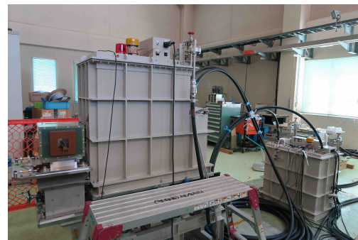
Figure 3: The injection kicker magnet with the magnetic switch tank and the thyratron tank.
