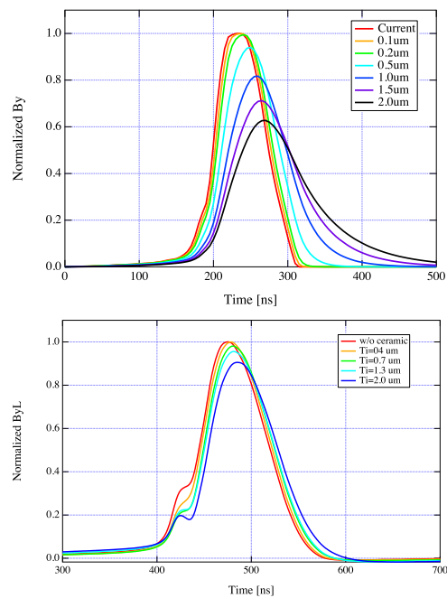
Figure 6: Magnetic fields by simulation (up) and experimental (down) results for a single pulse with various titanium coating thickness. The red line shows the fields from a case without the ceramic duct.
