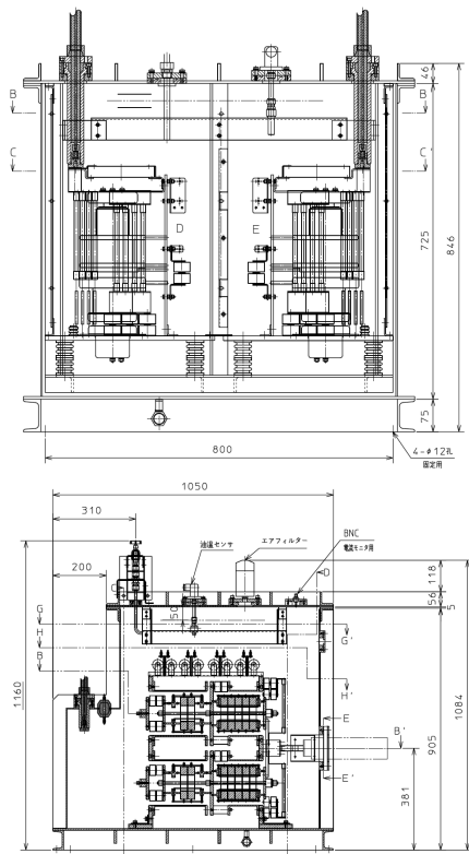
Figure 4: The drawing of the thyatron tank (up) and magnetic switch tank (down). Two thyratrons (e2V cx1836) are housed in a thyatron tank. The magnetic switch consists of four pulse transformers and four saturable inductances.
