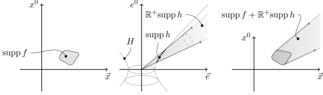
Figure 2.2.1: Localization region of a smeared string-field
