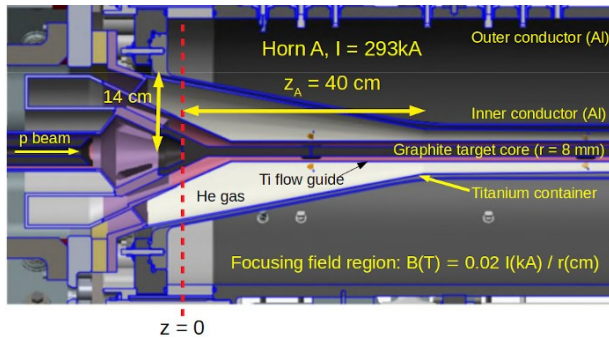
Figure 2: Layout of the target inside the first focusing horn.
