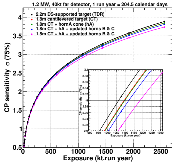
Figure 5: CP sensitivity \sigma versus exposure (detector mass times runtime) for different target-horn design iterations. The inset shows the zoomed-in region near \sigma = 3 .
