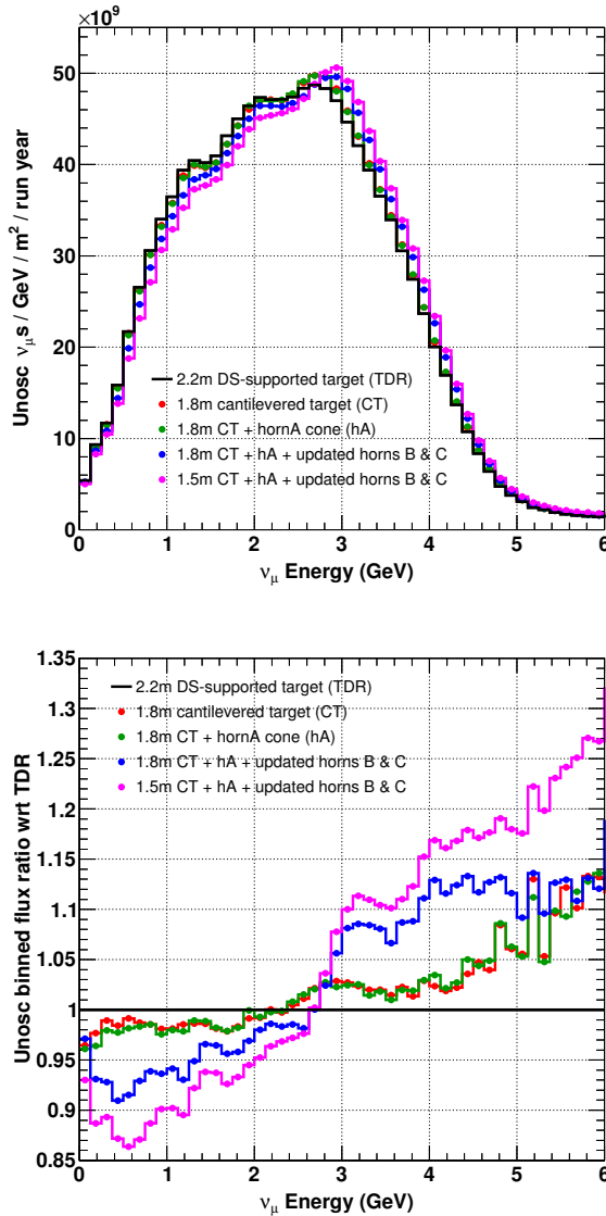
Figure 4: Top: unoscillated muon neutrino flux at the far detector for different target-horn design iterations. Bottom: Flux ratio with respect to the TDR design (2.2 m target).
