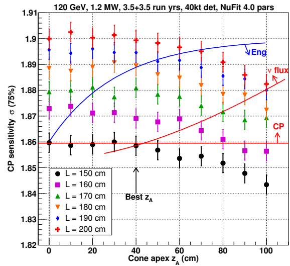
Figure 3: CP sensitivity \sigma versus the horn A upstream inner conductor cone apex z_A for different cantilever target core lengths. The blue and red curves indicate the engineering and physics (neutrino flux and CP \sigma ) limits, respectively.
