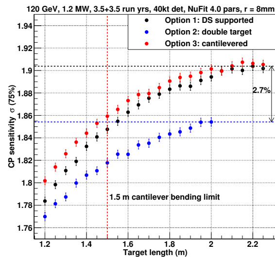
Figure 1: CP sensitivity \sigma (for 75% of the \delta_{CP} range) versus core target length for the 3 conceptual design options.
