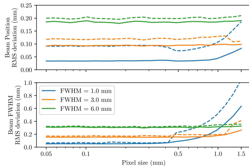
Figure 20. Uncertainty (RMS deviation) of reconstructed beam position (top) and beam width (bottom) of simulated frames as a function of pixel size [36]. Two algorithms are used: simple mean (dashed line) and likelihood fit of a Gaussian function (solid line). The beam is simulated by a random number of hits per frame following Poisson statistics and a Gaussian distribution with an insensitive gap of 300 \mu\text{m} at the edge of the beam. The pixel size is varied and three beam widths (different colors) are tested.
