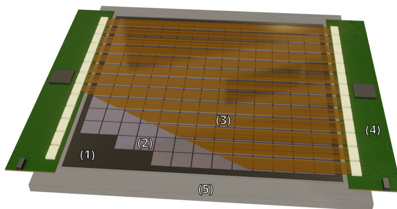
Figure 3. Schematic 3D rendering of the full size matrix with 13 \times 13 chips (2), interconnected by flex cables (3), assembled on a thin carbon fiber plate (1). The surrounding electronic boards (4) are mounted on a stabilizing frame (5).
