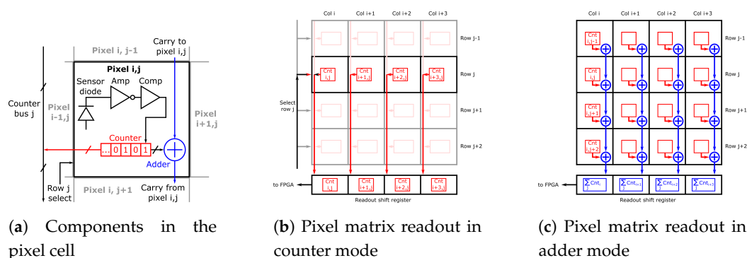
Figure 4. Illustration of the hit counting and adding features of the HitPix. In (a), the signal from the sensitive diode (Sensor diode) is amplified (Amp) and a threshold is applied in the comparator (Comp). The hits are counted and stored in the counter. This value can either be read out via the counter bus (left path in (a,b)), or added to the sum being propagated from the preceding pixel and then passed on to the next pixel (blue path in (a,c)).
