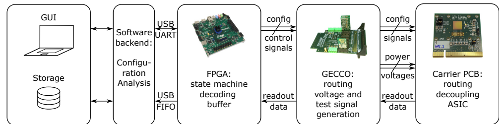
Figure 6. Block diagram of the data acquisition chain with the four components: PC, FPGA board, GECCO board and carrier board for the detector. Communication and data paths are indicated between the blocks.
