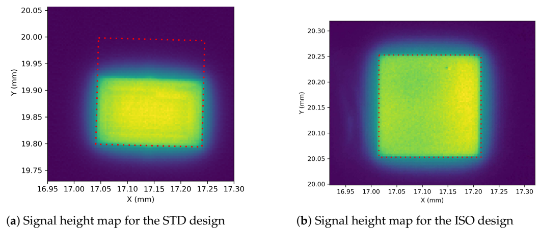
Figure 9. Signal height distribution measured on one pixel cell during illumination of the detectors with an infrared (904 nm) laser from the backside for the STD cell (a) and the ISO cell (b). The laser spot size was about 10 μm (FWHM) while the spatial step size was 1 μm. The setup is described in more detail in [37]. The analog signal of the pixel can be read out on a dedicated output line.
