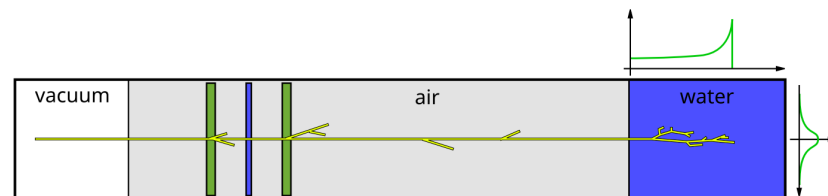
Figure 7. Illustration of the simulated setup. The green rectangles represent the position sensitive detectors and the narrow blue rectangle between them the effective water equivalent of the ionization chambers. The plots at the water box indicate examples of the expected transverse (top plot) and lateral (right plot) energy deposition.
