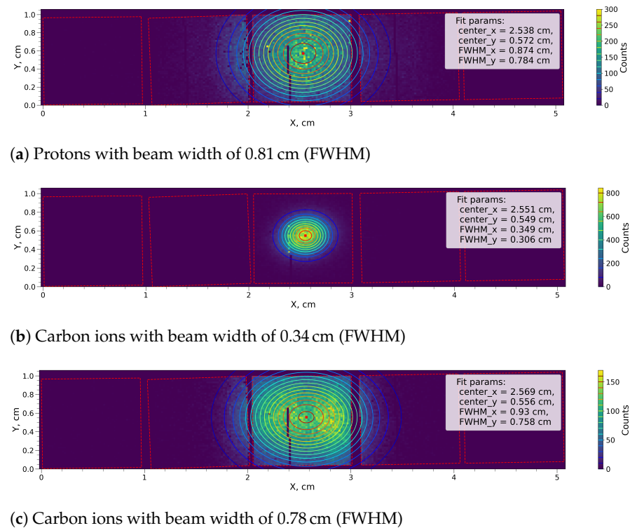
Figure 17. Hit maps for all five detectors of the matrix after alignment for three different beam settings. The red squares indicate the sensitive area of the aligned detectors. The colored circles are contour lines of the 2D Gaussian profile fitted to the hit distribution. The fit parameters are provided in the plots. Each plot contains about 250,000 hits.
