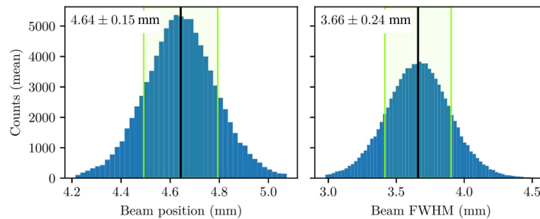
(c) Reconstructed beam centers (left) and beam widths (right) for a steady carbon ion beam for projected hit profiles from [36]. The integration time for a frame used for reconstruction was 30 \mu\text{s} .
