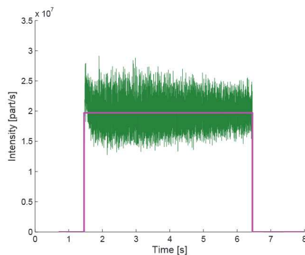
Figure 2. Time structure of a spill measured with an ionization chamber taken from [6]. The magenta line represents the desired spill shape, while the green line is the actual measurement. This example is for a carbon ion beam with 250 MeV/u; it can be different for other beam settings.
