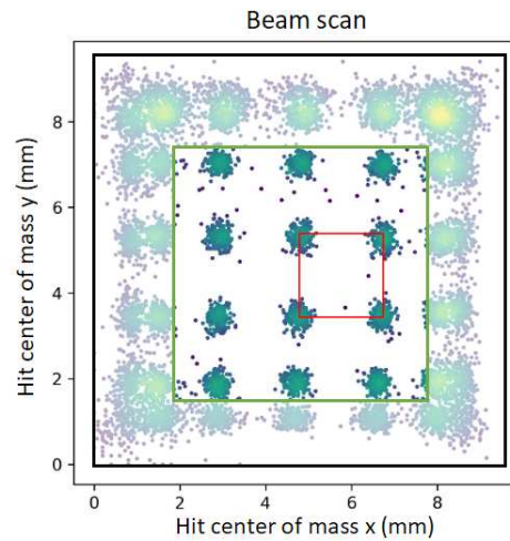
(a) Reconstructed beam centers for a continuous spot scan with 2 mm steps. The detector was in counter readout mode with 50 \mu\text{s} integration time per frame. Each point in the plot corresponds to the reconstructed beam center in a frame. The 2 mm raster is indicated by the red square. The green square indicates the area without distortions which occur at the edge of a single detector.
