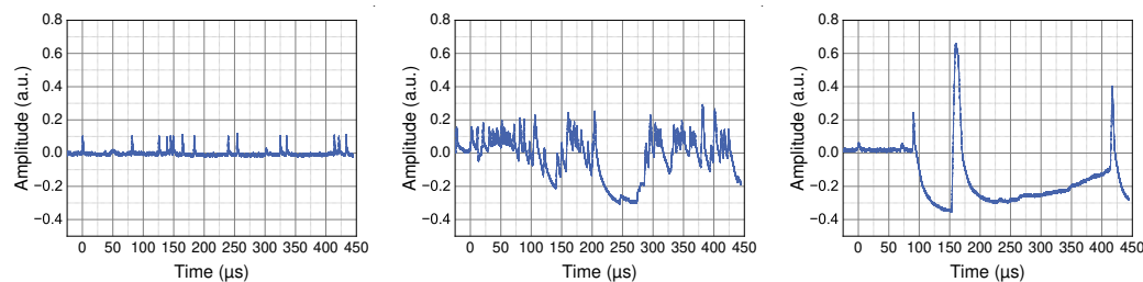
(a) Protons; beam intensity: 8 \times 10^7 \text{ s}^{-1} ; extrapolated local particle rate: 20 kHz. (b) Protons; beam intensity: 4 \times 10^8 \text{ s}^{-1} ; extrapolated local particle rate: 50 kHz. (c) Carbon ions; beam intensity: 2 \times 10^6 \text{ s}^{-1} ; extrapolated local particle rate: 250 Hz.
