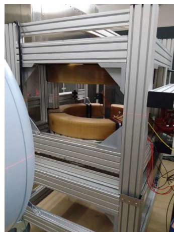
(a) Helmholtz coil pair
