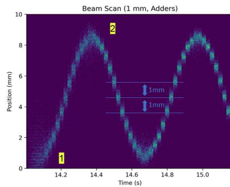
(b) Reconstructed beam centers for a continuous spot scan with 1 mm step size using adder readout with 20 \mu\text{s} integration time. Two features are indicated in the plot: at '1' the beam intensity ramps up, and at '2' part of the beam spot extends beyond the detector edge, which deteriorates the position reconstruction. In the center, the beam spot is contained within the detector matrix and a correct reconstruction is possible, showing the expected 1 mm steps.
