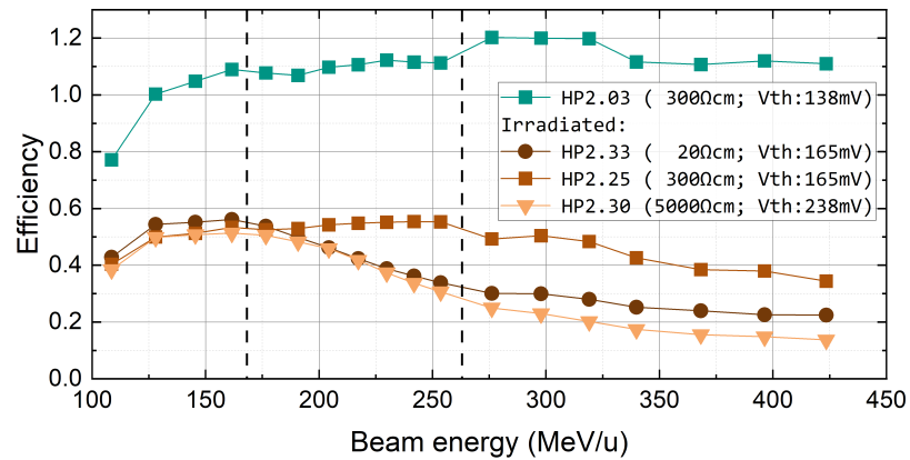
Figure 11. Hit detection efficiency measured with carbon ions of different energies after [36]. Sample HP2.03 (300 \Omega cm) is not irradiated and operated at 50 V, while the other samples are irradiated to a 1 MeV equivalent fluence of 1 \times 10^{15} \text{ cm}^{-2} and operated at 25 V. The two numbers in the brackets behind the sample name in the legend correspond to substrate resistivity and comparator threshold voltage ( V_{th} ), respectively. Beam parameters: carbon ions, 5 \times 10^6 \text{ s}^{-1}/3 \times 10^6 \text{ s}^{-1} particle rate for the unirradiated/irradiated sample, respectively, spot width adapted (steps indicated by vertical dashed lines) depending on the beam energy to stay at around 8 mm to 9 mm (FWHM).
