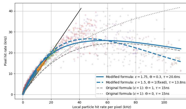
Figure 13. Single pixel hit rates versus expected local particle rates adapted from [36]. The plot combines data from spot irradiations with different beam intensities (colors: 5 \times 10^6\ \text{s}^{-1} (blue), 1 \times 10^7\ \text{s}^{-1} (orange), 2 \times 10^7\ \text{s}^{-1} (green), 3 \times 10^7\ \text{s}^{-1} (red), 5 \times 10^7\ \text{s}^{-1} (violet), 8 \times 10^7\ \text{s}^{-1} (brown)). For each pixel, the expected local particle rate is calculated assuming a Gaussian beam profile and the nominal beam intensities. The black line indicates a 100% hit detection efficiency. The solid blue line is a fit according to Equation (3) with \epsilon = 1.75 , \theta = 0.31 and \tau = 20.6\ \mu\text{s} . Forcing a fully paralyzing dead time (dashed blue line) fits the data better at higher rates. For comparison, the curves for the original Takecs formula are also provided (dashed gray: fully paralyzing; dotted gray: not paralyzing). Beam parameters: carbon ions, 430\ \text{MeV}/u energy, 3.4\ \text{mm} spot width (FWHM).
