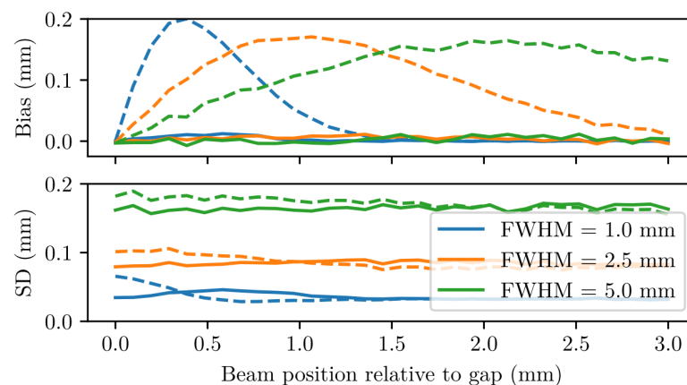
(b) Reconstructed beam position bias (top) and standard deviation (bottom) of simulated frames as a function of the distance to a 600\ \mu\text{m} wide insensitive gap. Two algorithms are used: simple mean (dashed line) and likelihood fit of a Gaussian function (solid line). The beam is simulated by a random number of hits per frame following Poisson statistics and a Gaussian distribution. The true beam position is varied and three beam widths (different colors) are tested.
