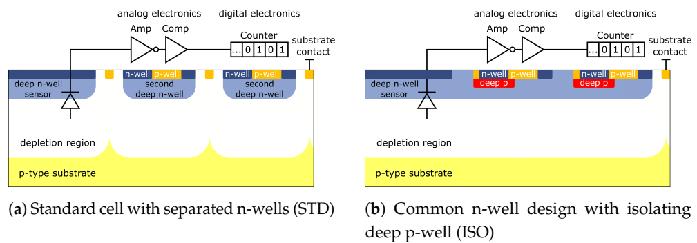
Figure 8. Pixel cross-sections of the two designs. In the STD design, the n-wells are separated from the charge collecting diodes and electronics (a). A common n-well enlarges the collecting diode, but requires deep p-wells to isolate the electronics (b). After [34].
