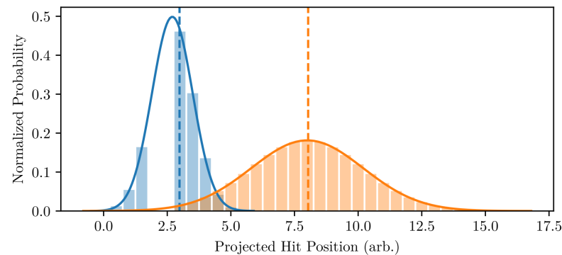
(a) Illustration of two simulated beam profiles with an insensitive gap at x = 2.5 . The vertical dashed lines represent the true center of the beams, and the solid lines a Gaussian fit of the hit counts represented by the bars. For the narrow beam, the bias of the reconstructed peak is visible. Statistical fluctuations are omitted for this example.
