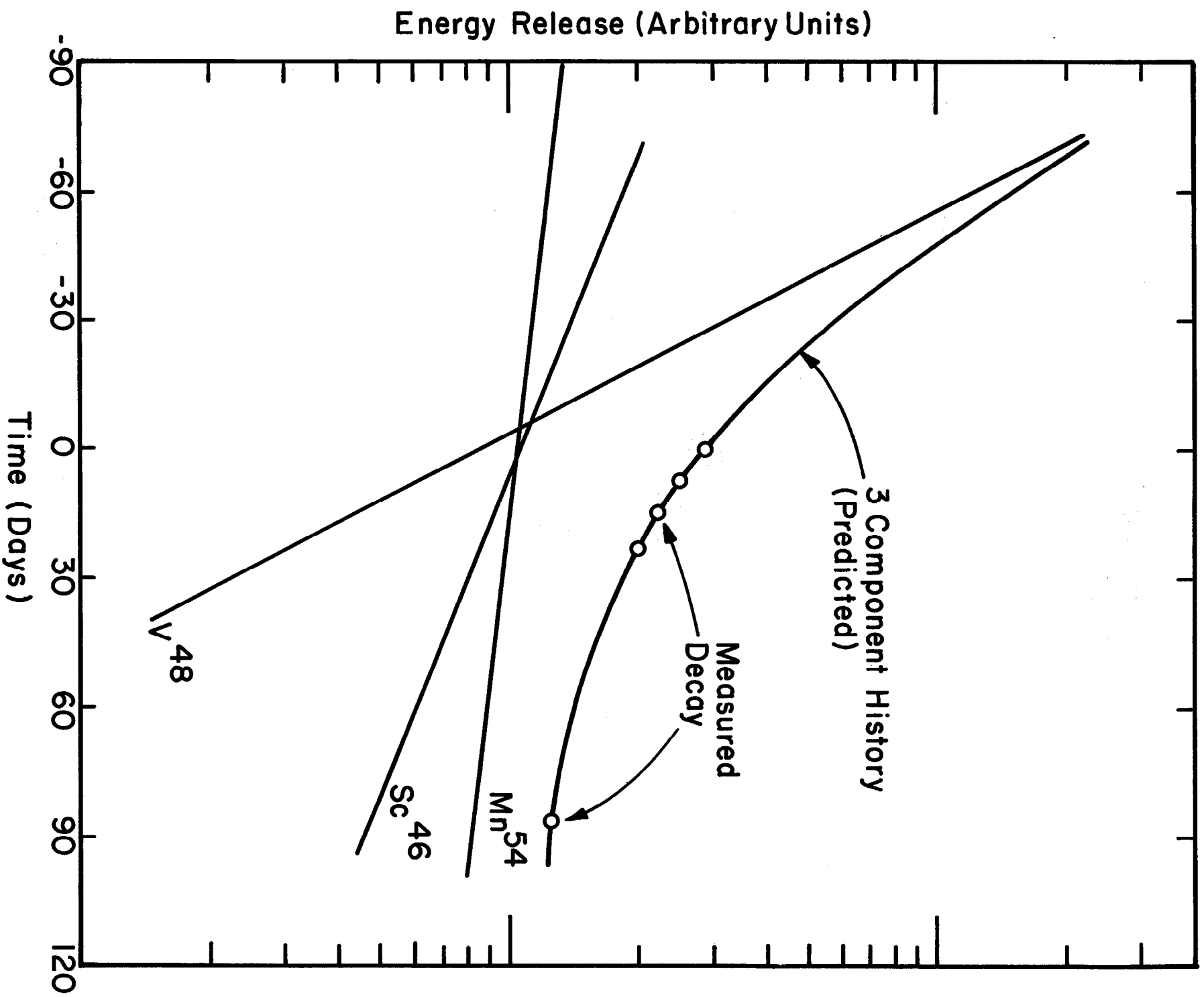
Fig. 5. Estimated radioactivity of dump as a function of time.
