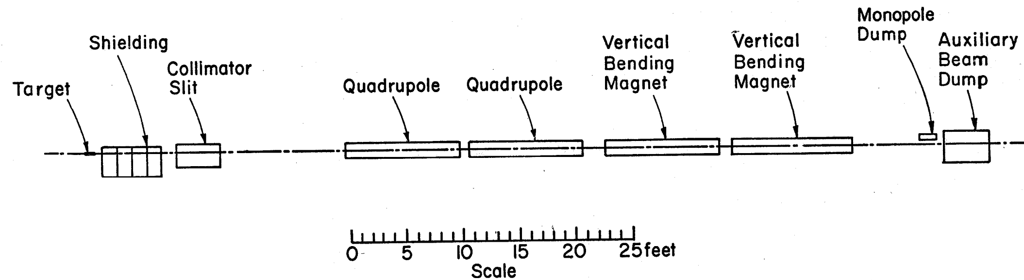
Figure 2 - Schematic of Dump Location in Nu-Hall
