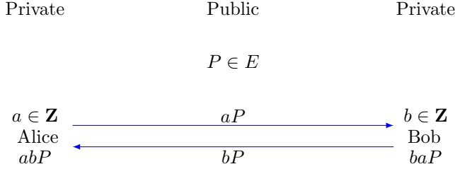
Figure 2.2: An Elliptic Curve Diffie–Hellman key-exchange.
