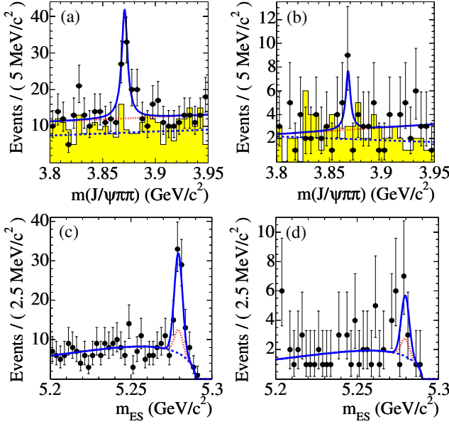
FIG. 1: Signal region projections of m(J/\psi \pi^+ \pi^-) and m_{ES} for B^- \rightarrow X(3872)K^- (a,c) and B^0 \rightarrow X(3872)K_s^0 (b,d). The dashed line represents the combinatorial background PDF, the dotted line represents the sum of the combinatorial and peaking background PDF, and the solid line the sum of all background plus the signal PDF. The shaded area shows events in the m_{ES} sideband region |m_{ES} - 5260 \text{ MeV}/c^2| < 6 \text{ MeV}/c^2 .
