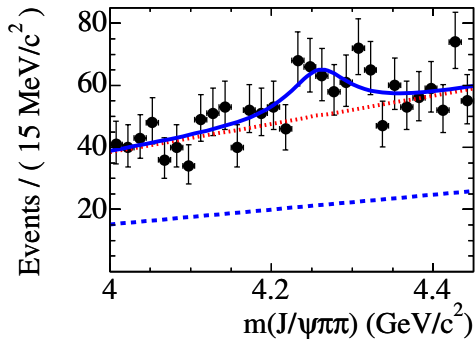
FIG. 2: Projection of the two-dimensional fit for the mass region above 4 \text{ GeV}/c^2 for events within the m_{\text{ES}} signal region in B^- \rightarrow J/\psi \pi^+ \pi^- K^- . The lines represent the same event types as in Fig. 1.
