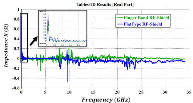
Figure 8: The comparison of transverse impedance in the X-direction.
