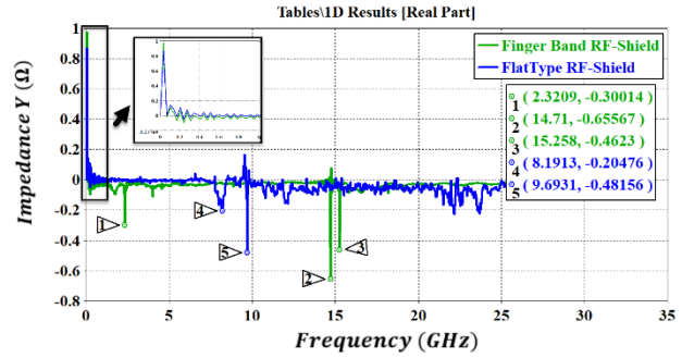
Figure 6: The comparison of transverse impedance in the Y-direction.
