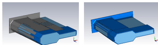
Figure 2: The Finger-Band (right) and the Flat-Type (left) geometry inside the Bellows.
