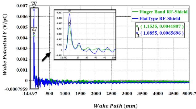
Figure 5: The comparison of transverse wake potential in the Y-direction.
