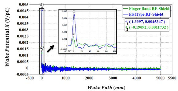
Figure 7: The comparison of transverse wake potential in the X-direction.
