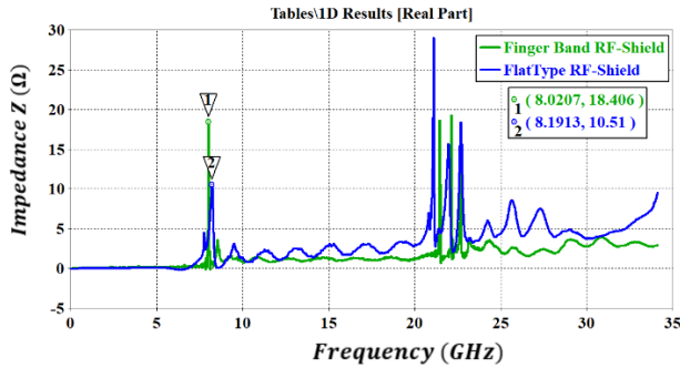
Figure 3: The comparison of longitudinal impedance in the Z-direction.
