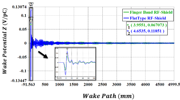
Figure 4: The comparison of longitudinal wake potential in the Z-direction
