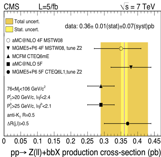
Figure 2. The inclusive Z+bb production cross section measurement compared with the theoretical expectations of the 4- and 5-flavour schemes tree level MADGRAPH calculations, the 5FS aMC@NLO, MCFM. Measurements are presented together with the relative statistical and statistical plus systematic uncertainty.
